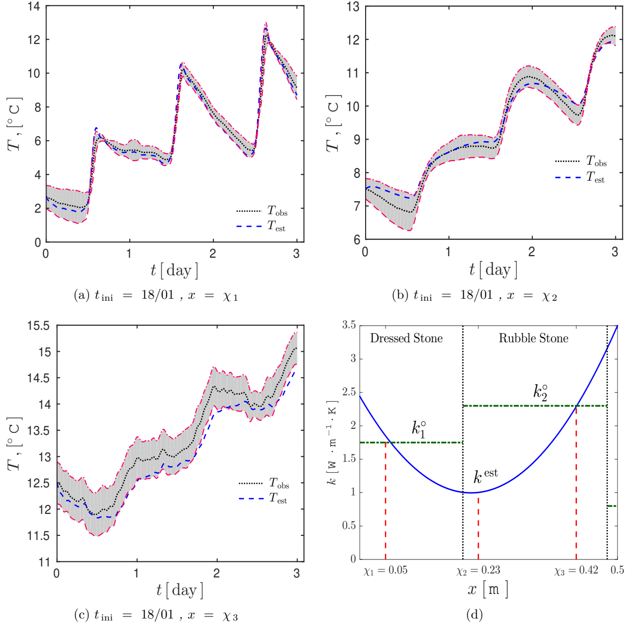
Figure 7. Variation of the computed temperature and the experimental observations for (a) first, (b) second and (c) third sensor locations; and (d) the estimated thermal conductivity representation.
