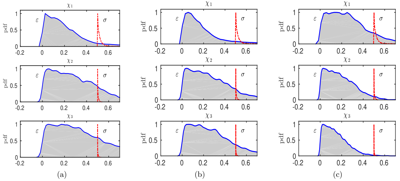
Figure 10. Normalized probability density function of the error distribution for the piecewise (a), linear (b), and quadratic (c) representations compared to the distribution of the measurement uncertainty \sigma values during one year for each sensor location.
