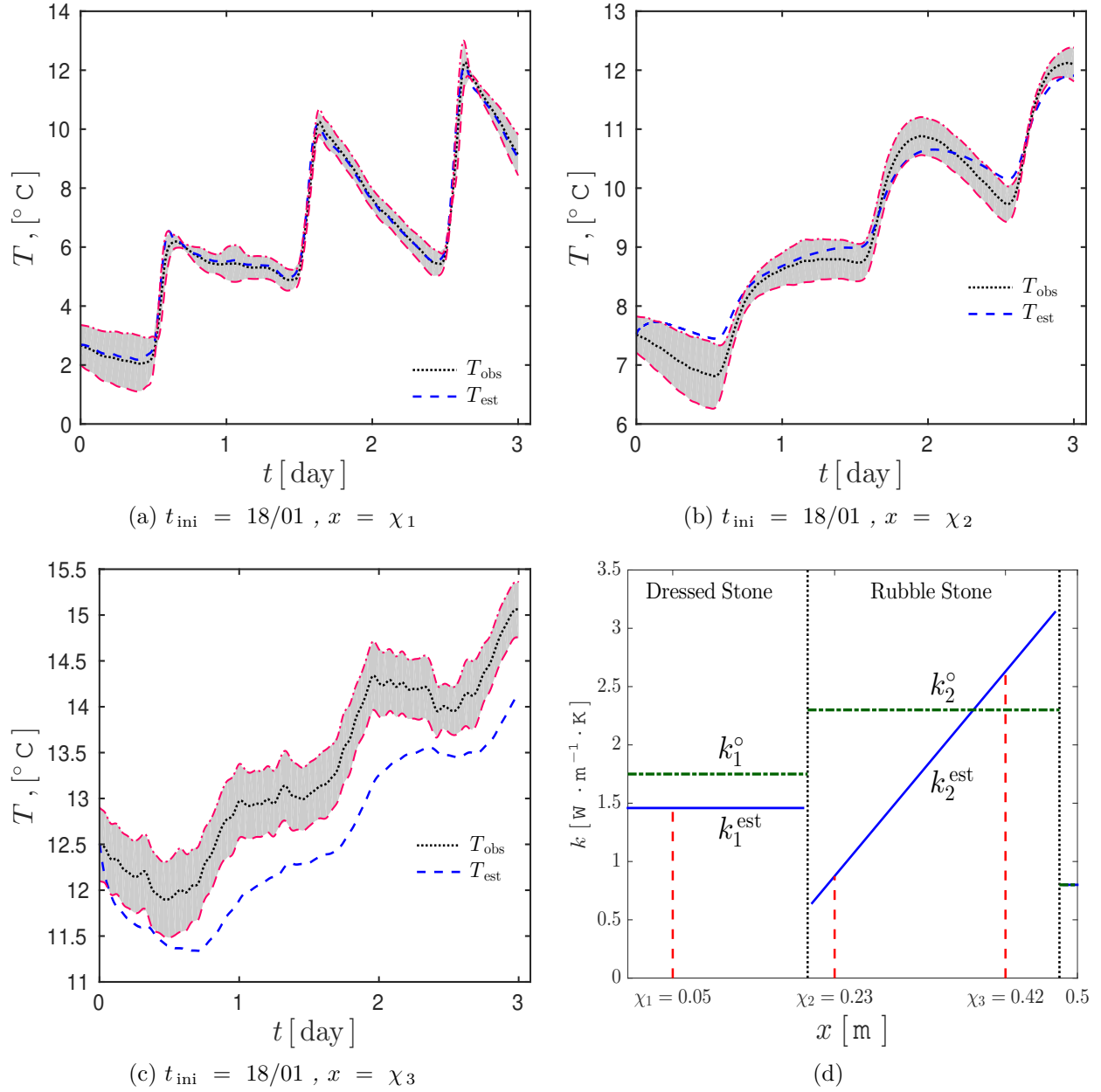
Figure 6. Variation of the computed temperature and the experimental observations for (a) first, (b) second and (c) third sensor locations; and (d) the estimated thermal conductivity representation.
