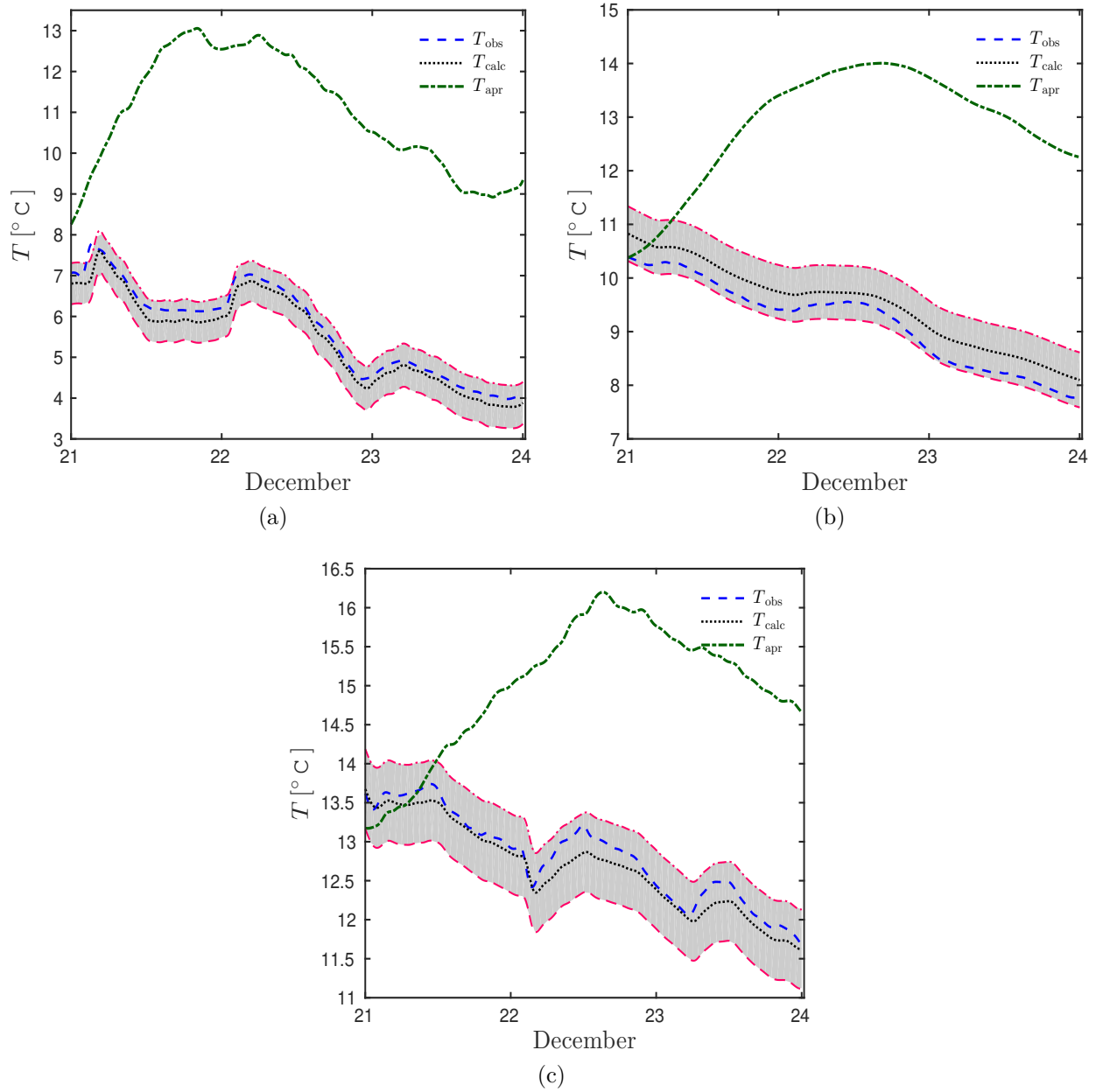
Figure 11. Variation of the a priori temperature, the computed temperature, and the experimental observations during the last three days of observations for (a) first, (b) second, and (c) third sensor locations.
