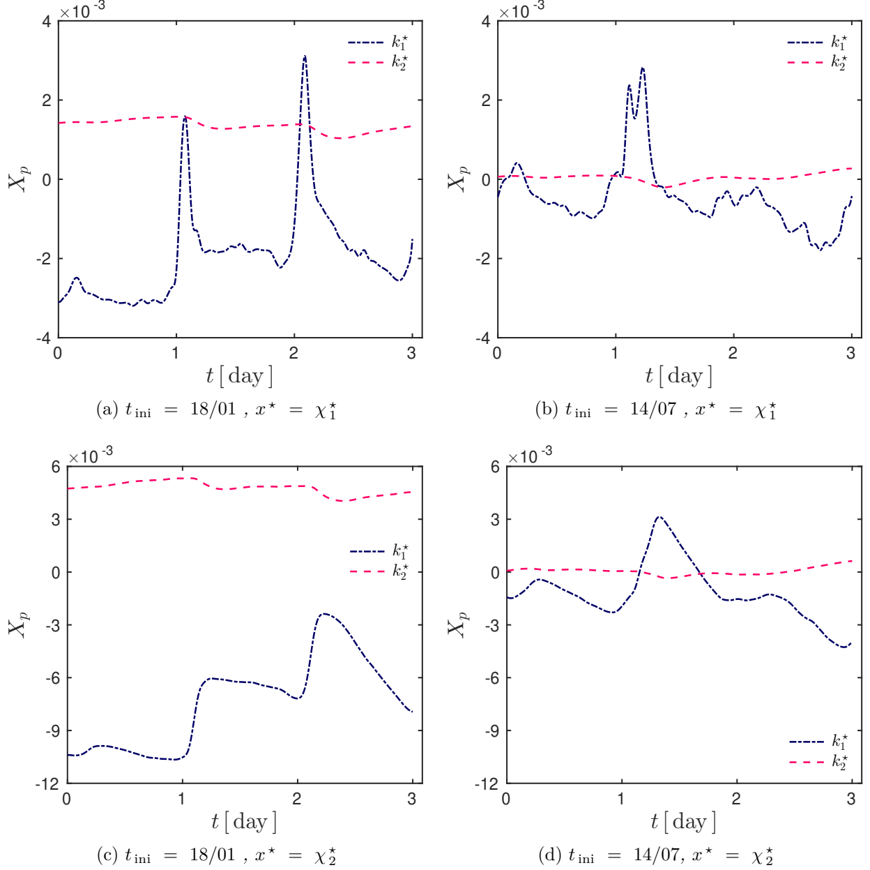
Figure 4. Variation of the sensitivity coefficients at the sensors location during 3 days in January and July.
