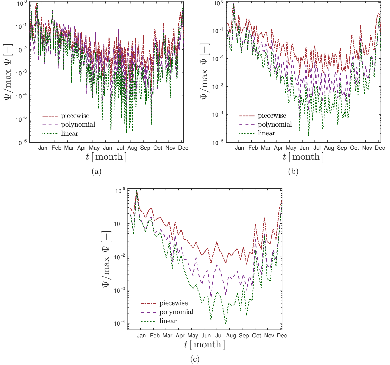
Figure 3. Variation of the criteria \Psi according to the length of observation period \delta\tau = 1 days (a), \delta\tau = 3 days (b) and \delta\tau = 7 days (c).
