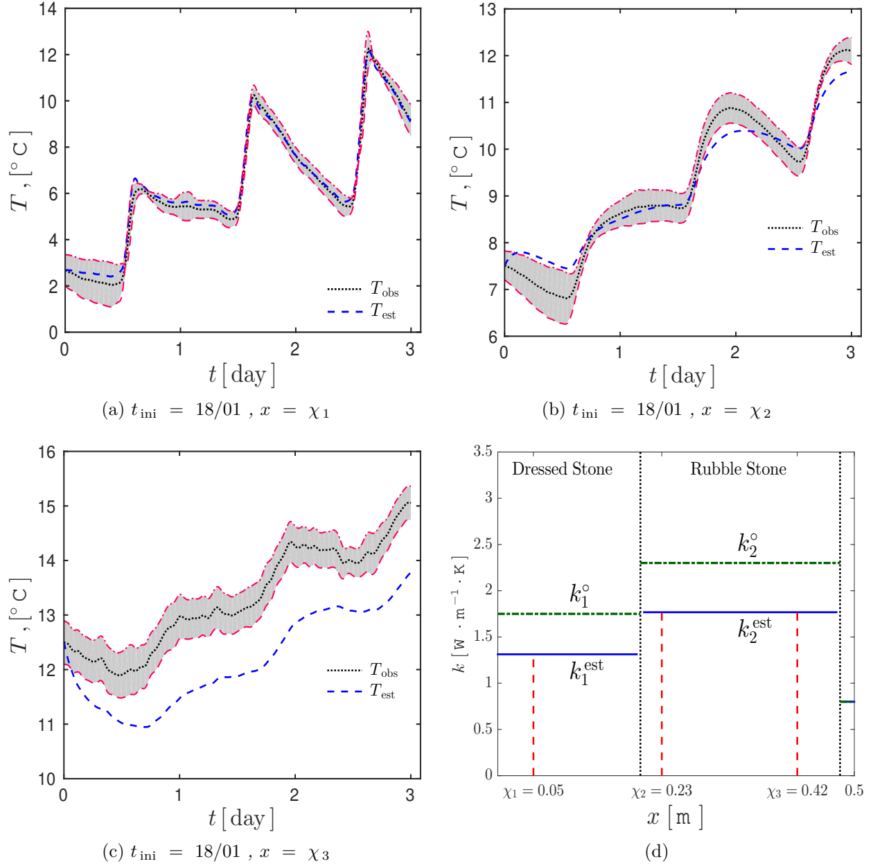
Figure 5. Variation of the computed temperature and the experimental observations for (a) first, (b) second and (c) third sensor locations; and (d) the estimated thermal conductivity representation.
