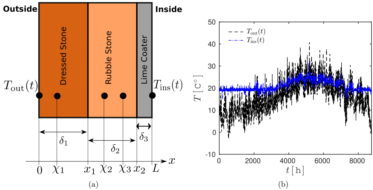
Figure 2. Illustration of the real case study (a) with the boundary conditions (b).
