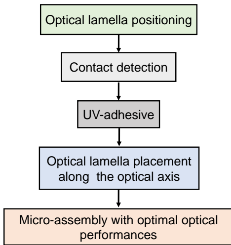
Fig. 1. The proposed micro-assembly task flowchart.
