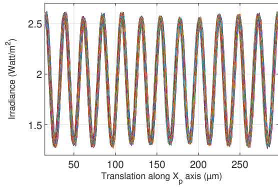
Fig. 15. Repeatability of the reflected light irradiance during experimentation for 30 translations.
