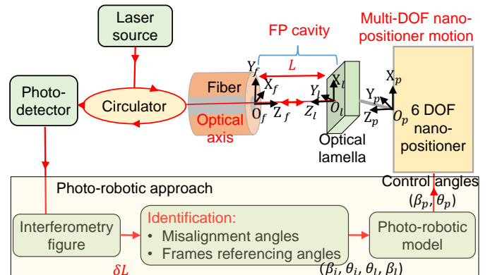
Fig. 5. The photo-robotic approach experimental implementation.
