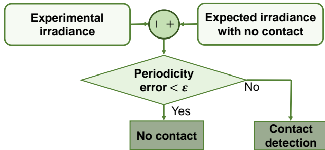
Fig. 16. Flowchart for contact detection based on FP interferometry measure.
