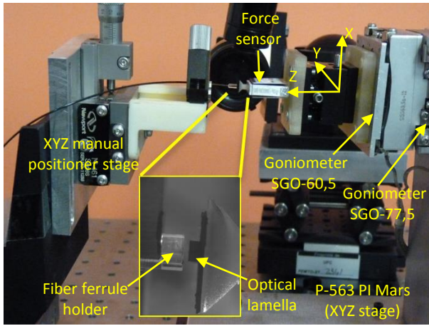
Fig. 3. Experimental setup: a 6 DOF nano-positioner used to move a photonic component in front of a fiber.
