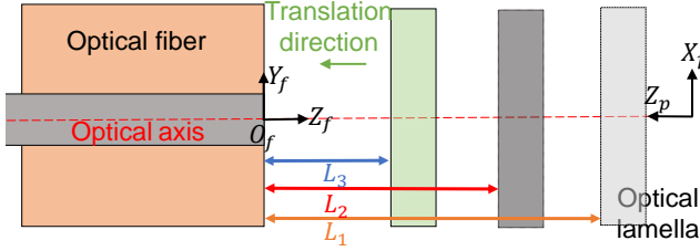
Fig. 6. Translation along the optical axis ( Z_f -axis) toward the fiber.
