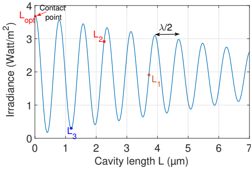
Fig. 7. Correlation between the FP cavity length L and a simulated FP interference for translation along the optical axis toward the fiber.
