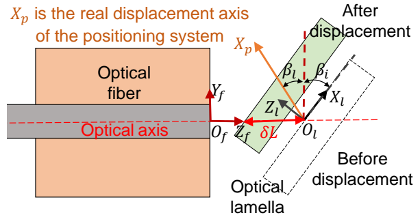
Fig. 4. Real displacement is along X_p and it is coupled with perpendicularity default angle \beta_i , frames referencing angle \beta_l and \delta L displacement along the optical axis.
