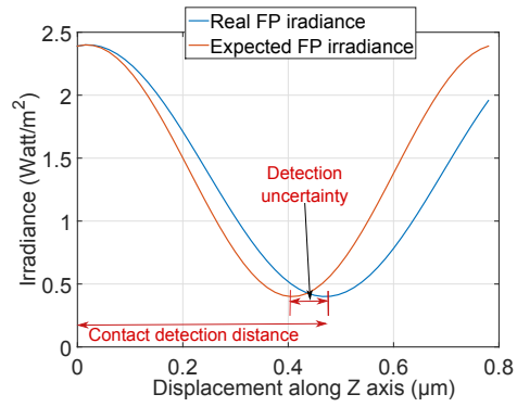
Fig. 14. Contact detection from expected and real FP irradiance periodicity difference.
