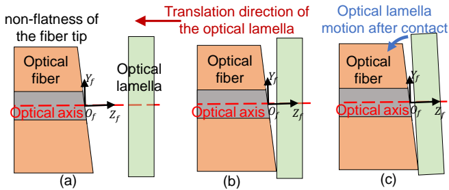
Fig. 13. (a) Optical lamella perpendicular to the optical axis (no contact), (b) Contact detection with zero force, (c) Contact with applied force (force estimation).
