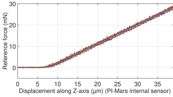
Fig. 10. The corresponding experimental sensed force for 7 forth motion along the Z-axis.
