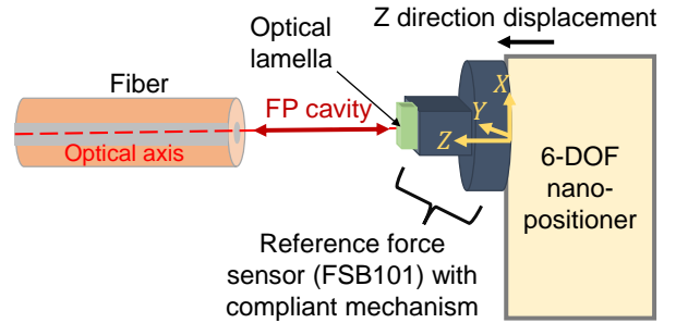
Fig. 9. Experimental set-up scheme for force estimation and contact detection.
