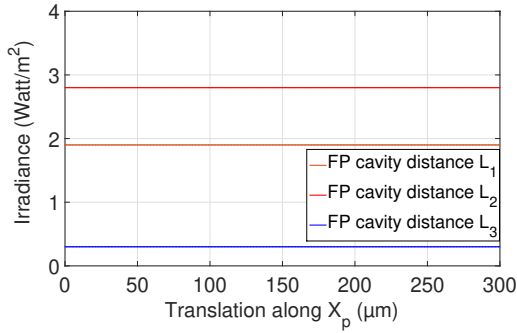
Fig. 8. The optical irradiance simulation corresponding to different FP cavity length when translating along X_p -axis.
