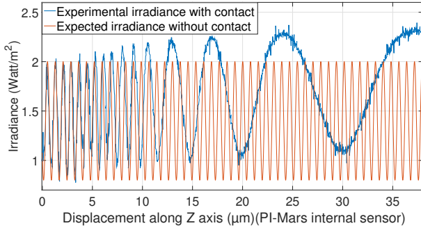
Fig. 11. Experimental FP interferences evolution when the photonic component is translated along the optical axis, a contact occurs at Z = 6.16 \mu\text{m} .
