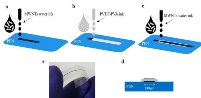
FIGURE 1. (a) Bottom electrode printed on PEN substrate using CNT water ink. (b) PVDF-PVA ink printed on the top of the bottom electrode, serving as a dielectric layer. The mass ratio between PVDF and PVA in the inks is 93:7. (c) Printing top CNT electrode on top of the dielectric layer. (d) Lateral view of the designed microcapacitor with an effective electrode width of around 140 \mu\text{m} . (e) Photograph of bent microcapacitor with an effective area of \sim 2.8 \times 10^{-6} \text{ m}^2 .
