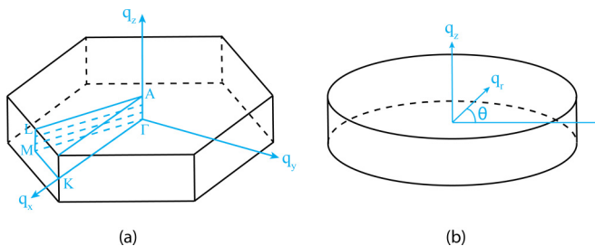
FIG. 2. Approximation of the first Brillouin zone (BZ) of graphite: (a) the realistic hexagonal first BZ and (b) the approximate cylindrical first BZ for solving Eq. (6). The dashed light blue lines within \Gamma ALM in (a) denote the discrete directions parallel to \Gamma-M at different q_z from \Gamma to A points.
