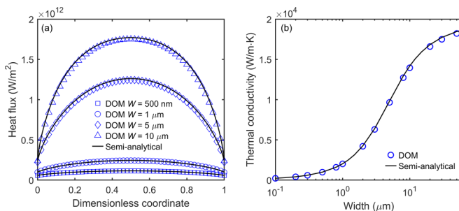
FIG. 5. Heat transport along an infinitely long graphite ribbon with a finite width at 100 K: (a) cross-sectional heat flux profile at different widths ( W ) and (b) width-dependent thermal conductivity. The discrete symbols denote the present discrete-ordinate method (DOM) solution, whereas the solid lines denote the semi-analytical solution from Ref. [26]. Isotopically pure graphite is considered, and a temperature gradient of -10^8 K/m is exerted.
