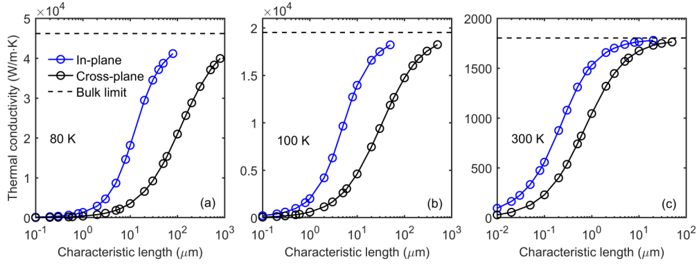
FIG. 7. Thermal conductivity of in-plane and cross-plane heat transport along infinitely long and infinitely wide graphite ribbons, respectively, at different temperatures: (a) 80 K, (b) 100 K, and (c) 300 K. Isotopically pure graphite is considered here, and the characteristic length denotes the width for the in-plane case or the length for the cross-plane case (c.f. Fig. 6).
