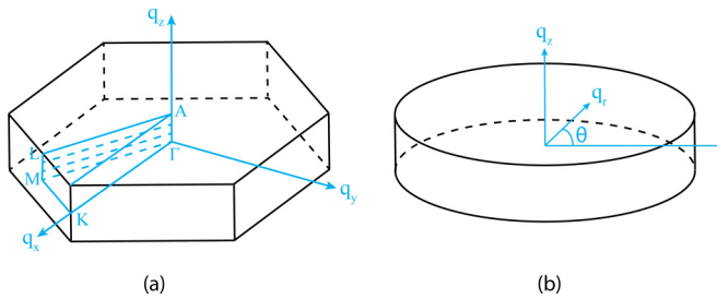
FIG. 2. Approximation of the first Brillouin zone (BZ) of graphite: (a) the realistic hexagonal first BZ and (b) the approximate cylindrical first BZ for solving Eq. (6). The dashed light blue lines within \Gamma ALM in (a) denote the discrete directions parallel to \Gamma-M at different q_z from \Gamma to A points.
