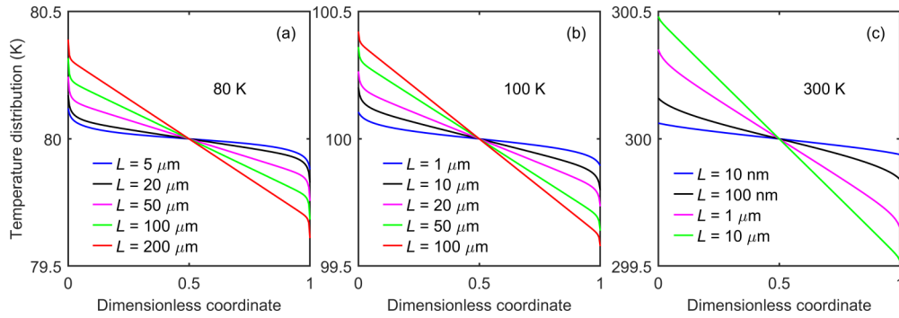
FIG. 9. Temperature distribution of cross-plane heat transport along an infinitely wide graphite ribbon with different lengths ( L ) at several temperatures: (a) 80 K, (b) 100 K, and (c) 300 K. Isotopically pure graphite is considered here.
