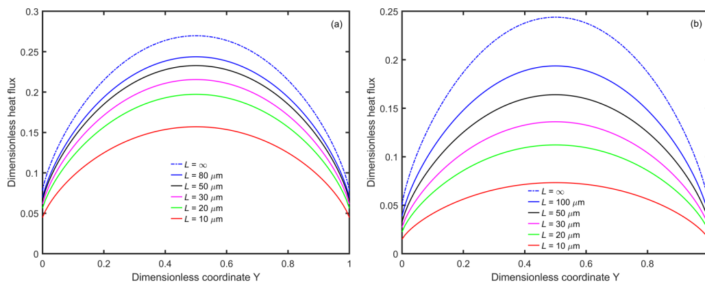
FIG. 13. The middle cross-sectional dimensionless heat flux profile of heat transport in rectangular graphite ribbons with different lengths ( L ): (a) W = 2 \mu\text{m} , 100 K; and (b) W = 5 \mu\text{m} , 80 K. Isotopically pure graphite is considered here, and the heat flux is normalized by the bulk limit.
