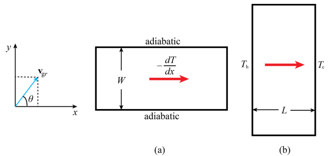
FIG. 6. Schematics of heat transport in the basal plane of the graphite ribbon: (a) in-plane heat transport along an infinitely long graphite ribbon with a finite width W and (b) cross-plane heat transport along an infinitely wide graphite ribbon with a finite length L .
