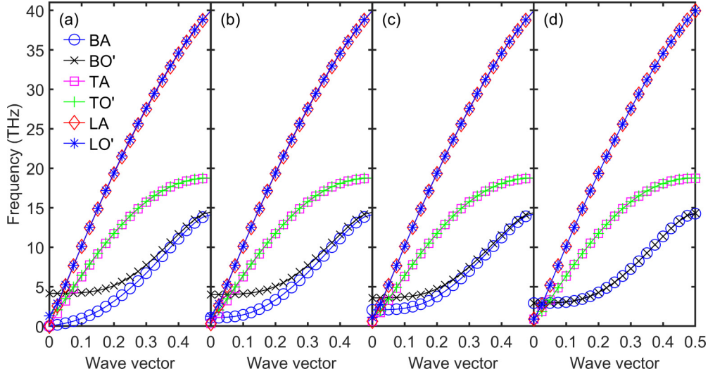
FIG. 15. Phonon dispersion of graphite at different dimensionless q_z from \Gamma to A points in the first Brillouin zone: (a) Q_z = 0 , (b) Q_z = \frac{1}{6} , (c) Q_z = \frac{1}{3} , and (d) Q_z = \frac{1}{2} . Six phonon branches along the \Gamma - M direction for Q_z = 0 and along the directions parallel to \Gamma - M within \Gamma ALM for other Q_z [c.f. Fig. 2(a)] are shown.
