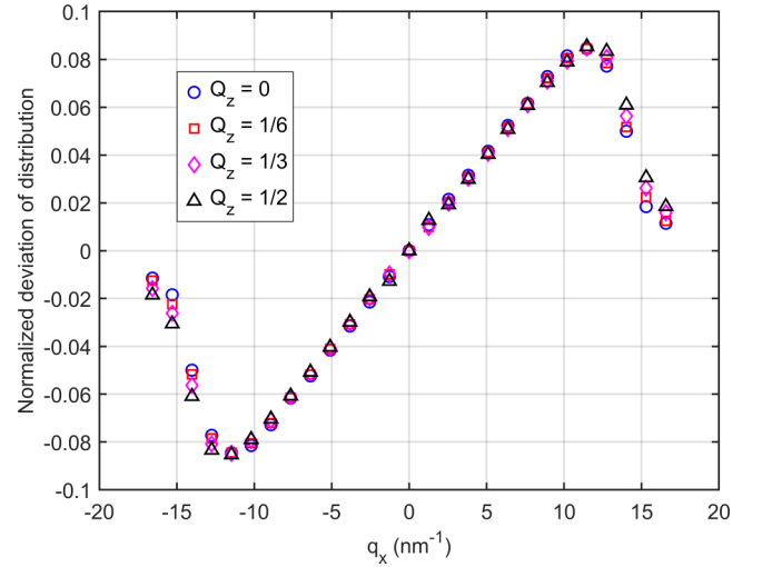
FIG. 14. Normalized deviation of distribution for bending acoustic (BA) phonons in isotopically pure graphite at 100 K at different dimensionless q_z from \Gamma to A points in the first Brillouin zone. The results are obtained through an iterative solution of phonon Boltzmann equation with the full scattering term. A temperature gradient of [-10^8 \ 0 \ 0] (K/m) is applied. The results at q_y = 0 are shown.
