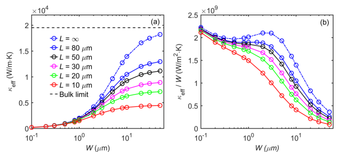
FIG. 11. (a) Width-dependent thermal conductivity and (b) normalized thermal conductivity of rectangular graphite ribbons with different lengths ( L ) at 100 K. Isotopically pure graphite is considered here, and the thermal conductivity normalized by the width ( W ) in (b) denotes the normalization by the ballistic limit.
