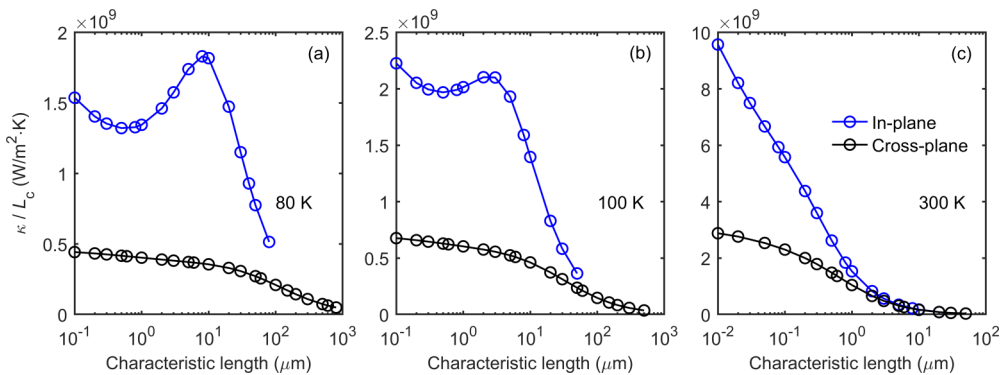
FIG. 8. Normalized thermal conductivity of in-plane and cross-plane heat transport along infinitely long and infinitely wide graphite ribbons, respectively, at different temperatures: (a) 80 K, (b) 100 K, and (c) 300 K. Isotopically pure graphite is considered here, and the characteristic length ( L_c ) denotes the width for the in-plane case or the length for the cross-plane case (c.f. Fig. 6). The thermal conductivity normalized by the characteristic length denotes a normalization by the ballistic limit.
