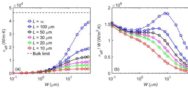
FIG. 12. (a) Width-dependent thermal conductivity and (b) normalized thermal conductivity of rectangular graphite ribbons with different lengths ( L ) at 80 K. Isotopically pure graphite is considered here, and the thermal conductivity normalized by the width ( W ) in (b) denotes the normalization by the ballistic limit.
