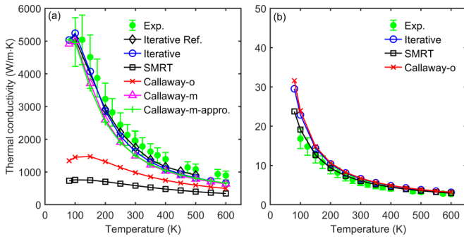
FIG. 16. Temperature-dependent bulk thermal conductivity of graphite with natural abundance (1.1% ^{13}\text{C} ): (a) basal plane result and (b) c -axis result. The line with circles denotes the iterative solution of phonon Boltzmann equation with full scattering term; the line with squares denotes the single mode relaxation time (SMRT) approximation; the line with cross symbols (or triangles) denotes the Callaway's dual relaxation model with the original (-o) definition [or modified (-m) definition in Eq. (13)] of normal and Umklapp scattering rates, whereas the line with plus symbols denotes the Callaway's model with the modified definition of normal and Umklapp scattering rates under the approximations made in Sec. II B 3. The line with diamonds refers to the iterative solution from Ref. [35] with the same pseudopotential and van der Waals (vdW) functional. The discrete filled circles with error bars denote the experimental results from Ref. [60].
