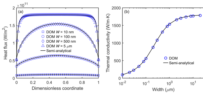
FIG. 4. Heat transport along an infinitely long graphite ribbon with a finite width at 300 K: (a) cross-sectional heat flux profile at different widths ( W ) and (b) width-dependent thermal conductivity. The discrete symbols denote the present discrete-ordinate method (DOM) solution, whereas the solid lines denote the semi-analytical solution from Ref. [26]. Isotopically pure graphite is considered, and a temperature gradient of -10^8 K/m is exerted.
