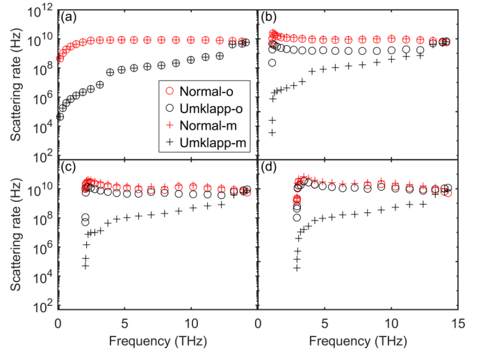
FIG. 1. Normal and Umklapp scattering rates of bending acoustic (BA) phonons in isotopically pure graphite at 100 K at different dimensionless q_z from \Gamma to A points in the first Brillouin zone: (a) Q_z = 0 , (b) Q_z = \frac{1}{6} , (c) Q_z = \frac{1}{3} , and (d) Q_z = \frac{1}{2} . The red and black circles (or plus symbols) denote, respectively, the normal and umklapp scattering rates based on the original (-o) definition [or modified (-m) definition in Eq. (13)]. The representative results along the \Gamma - M direction for Q_z = 0 and along the directions parallel to \Gamma - M within \Gamma ALM for other Q_z [c.f. Fig. 2(a)] are shown.
