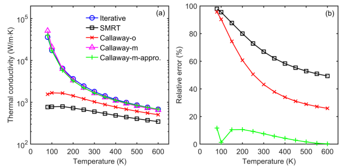
FIG. 3. Temperature-dependent bulk thermal conductivity of isotopically pure graphite: (a) basal plane result and (b) relative error of the relaxation approximations comparing with the iterative solution. The line with circles denotes the iterative solution of the phonon Boltzmann equation with a full scattering term; the line with squares denotes the single mode relaxation time (SMRT) approximation; the line with cross symbols (or triangles) denotes the Callaway's dual relaxation model with the original (-o) definition [or modified (-m) definition in Eq. (13)] of normal and Umklapp scattering rates, whereas the line with plus symbols denotes the Callaway's model with the modified definition of normal and Umklapp scattering rates under the approximations made in Sec. II B 3.
