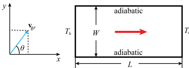
FIG. 10. Schematic of heat transport along a graphite ribbon with a finite length L and a finite width W .
