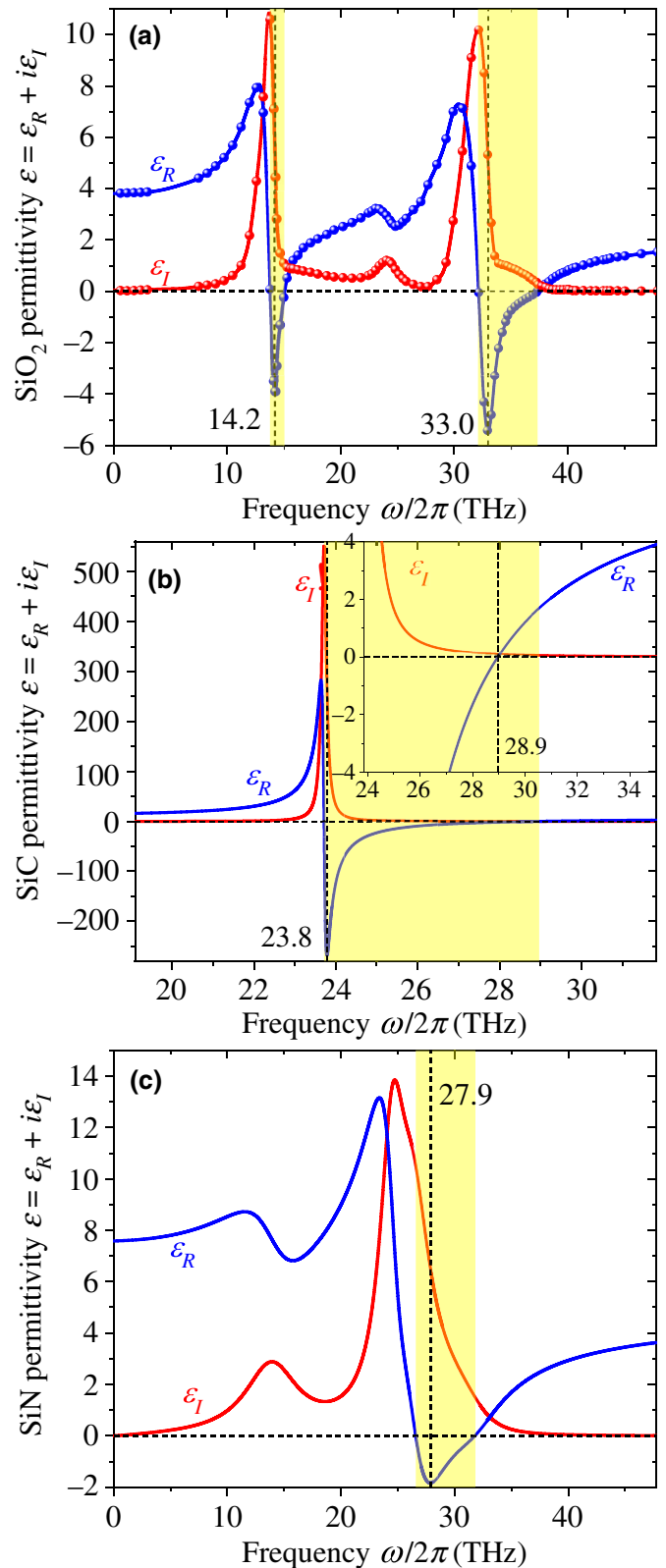
FIG. 3. Real and imaginary parts of the relative permittivity \varepsilon(\omega) = \varepsilon_R(\omega) + i\varepsilon_I(\omega) of (a) SiO 2 , (b) SiC, and (c) SiN as a function of frequency [2,3,5]. The yellow zones stand for the Reststrahlen bands [ \varepsilon_R(\omega) < 0 ] of each material.
