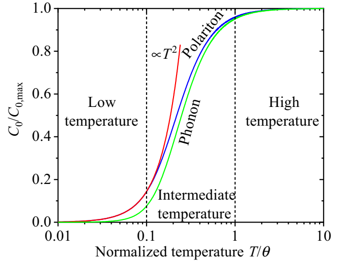
FIG. 2. Fundamental component of the SPHP heat capacity of a polar nanofilm as a function of its temperature. The red line represents the low-temperature limit predicted by Eq. (9) and the green one stands for the prediction of the Debye model for phonons.
