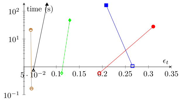
Figure 4: (Top) Runtime vs. classification error ( \epsilon_t ) for multi-task multi-class MTL-LSSVM (filled marks) and MTL-SPCA (empty marks). (Bottom) Datasets. Synthetic: \mu_j = 2e_j^{[p]} , \mu_j^\perp = 2e_{p-j}^{[p]} , \beta_1 = 0.2 , \beta_2 = 0.4 , \beta_3 = 0.6 ; p = 200 , n_{1j} = n_{2j} = 100 , n_{3j} = 50 ; 1000 test sample averaging.
