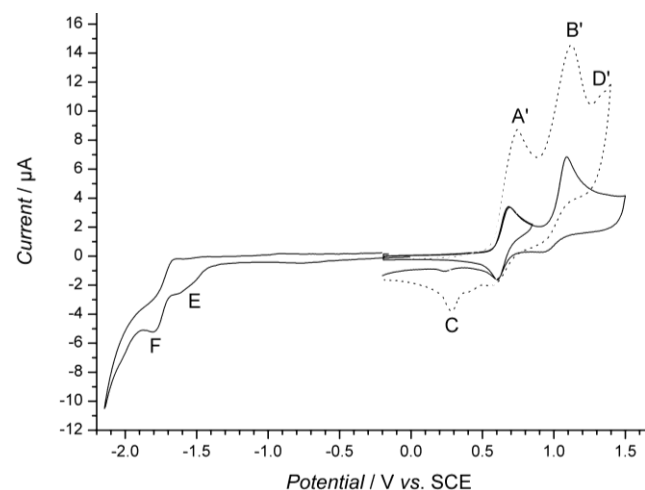
Fig. 2 Cyclic voltammograms of 1 in CH 2 Cl 2 with TBAP 0.1 M. Concentration: 5 \times 10 -4 (solid line) and 10 -3 M (dotted line); WE: Pt \phi = 2 mm, scan rate: \nu = 100 mV s -1 ; initial potential = -0.20 V.
