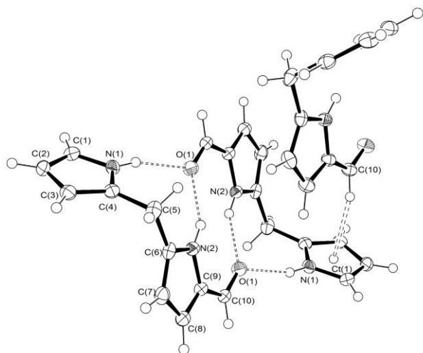
Fig. 1 Ortep 15 view of three 1-formyldipyrromethane ( 2 ) asymmetric units. The thermal ellipsoids are at the 50% probability level. Hydrogen bonds and CH... \pi interactions are indicated by dashed lines.
