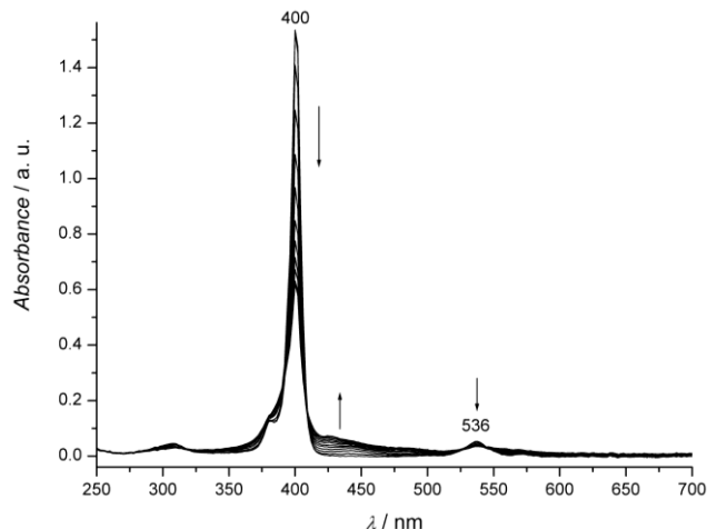
Fig. 3 Electrolysis of a 1.8 \times 10^{-5} \text{ M} solution of 1 followed by UV-Vis spectroscopy ( l = 2 \text{ mm} , 0.1 \text{ M} TBAP in \text{CH}_2\text{Cl}_2 , E_{\text{app}} = 0.70 \text{ V vs. SCE} , -1 electron, WE: Pt wire).
