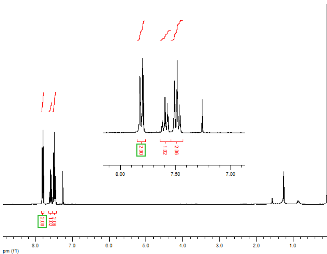
Figure S14. 1 H NMR spectra (CDCl 3 ) for photo-produced Bzp-H from Bzp-Br. Top: crude. Bottom: same batch after purification on silica chromatography.
