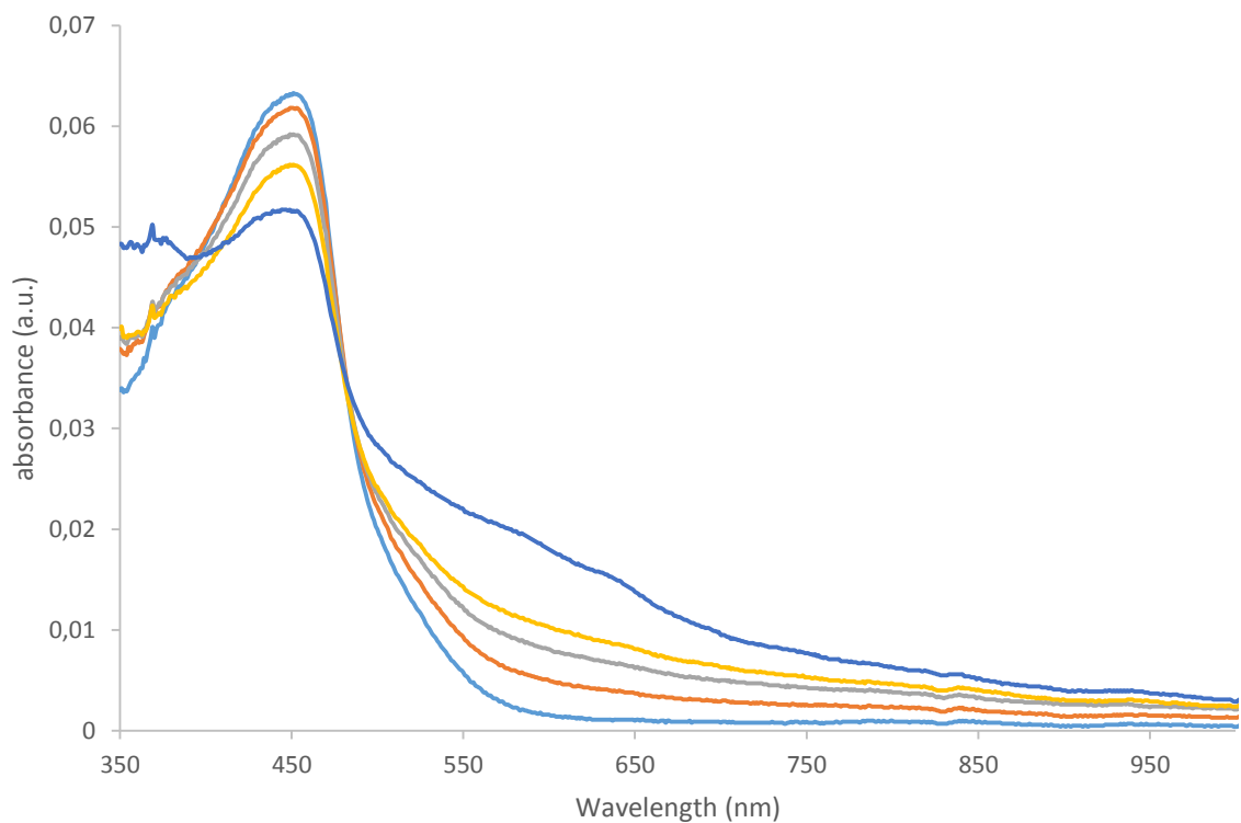
Figure S10. Evolution of the UV-Vis spectra of C1 in THF upon reduction (supporting electrolyte: tetrabutylammonium hexafluorophosphate 0.1 M).
