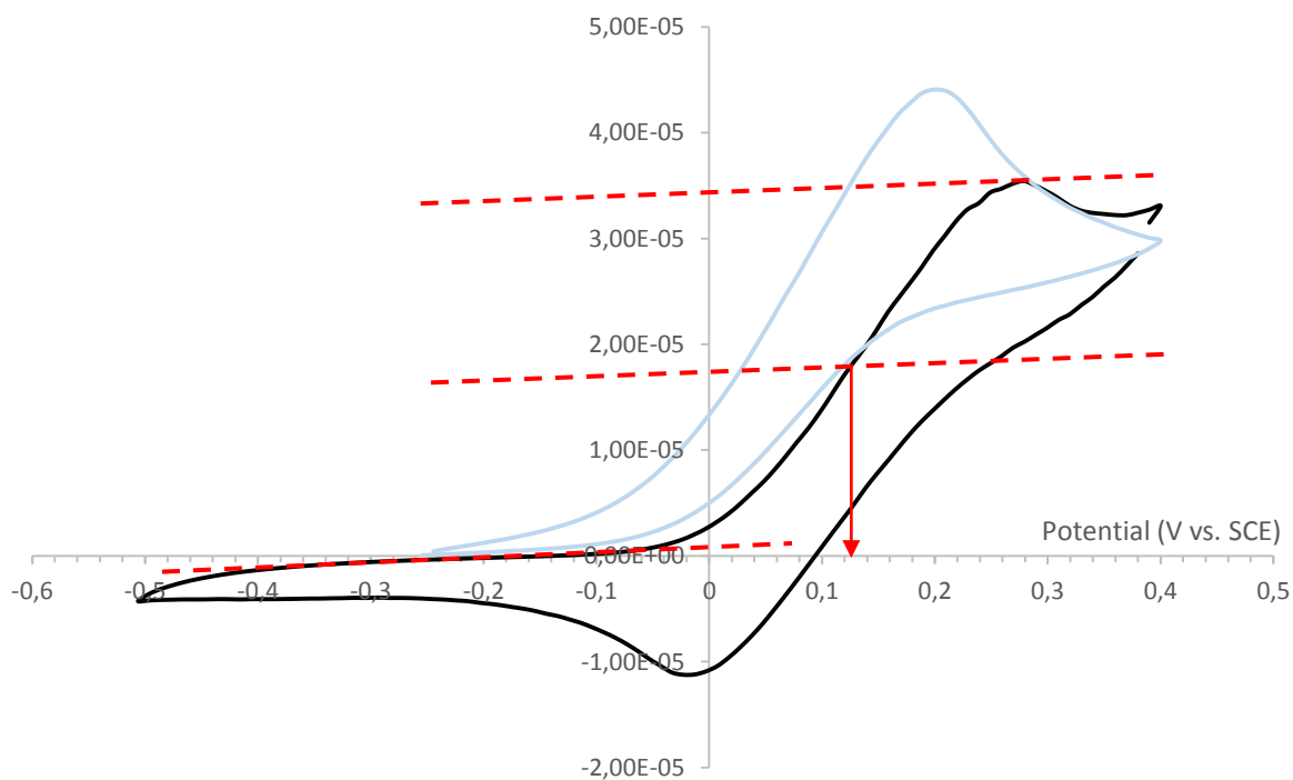
Figure S5. Cyclic voltamperometry of BI 2 H in THF (black line) and in presence of 1 equivalent of TEA (blue line) with glassy carbon as working electrode, platinum grid for counter electrode and SCE for the reference electrode.
