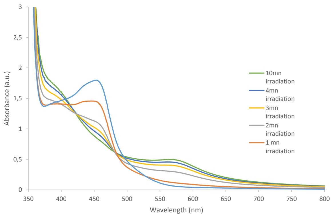
Figure S8. Evolution of the UV-Vis spectra of C1 , BI 1 H and TEA in deaerated acetonitrile under irradiation at 450 nm (blue LED).
