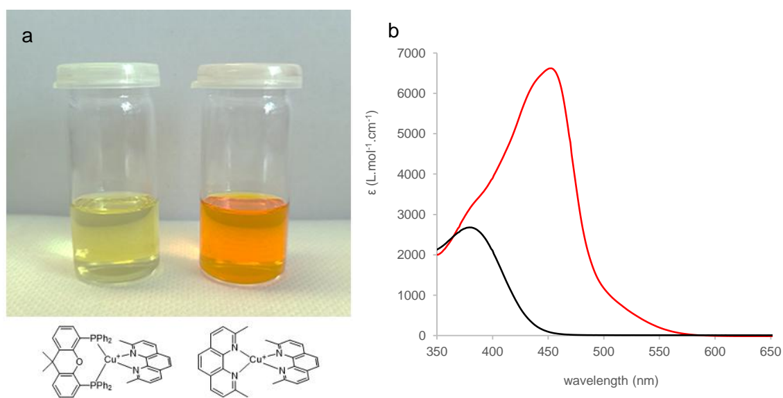
Figure S1. (a) Weakly colored but strong photo-oxidant heteroleptic vs. strongly colored but weakly photo-oxidant homoleptic Cu(I) complexes (0.1 mM solutions in dichloromethane). In this picture, complexes with G = methyl (left: C2 : [\text{Cu}(\text{xantphos})(\text{dmp})]^+ , dmp = 2,9-dimethyl-1,10-phenanthroline. Right: [\text{Cu}(\text{dmp})_2]^+ ) have been chosen to illustrate the color differences. (b) Absorption spectra of [\text{Cu}(\text{XantPhos})(\text{dmp})]^+ and [\text{Cu}(\text{dmp})_2]^+ ( C1 ) in THF.
