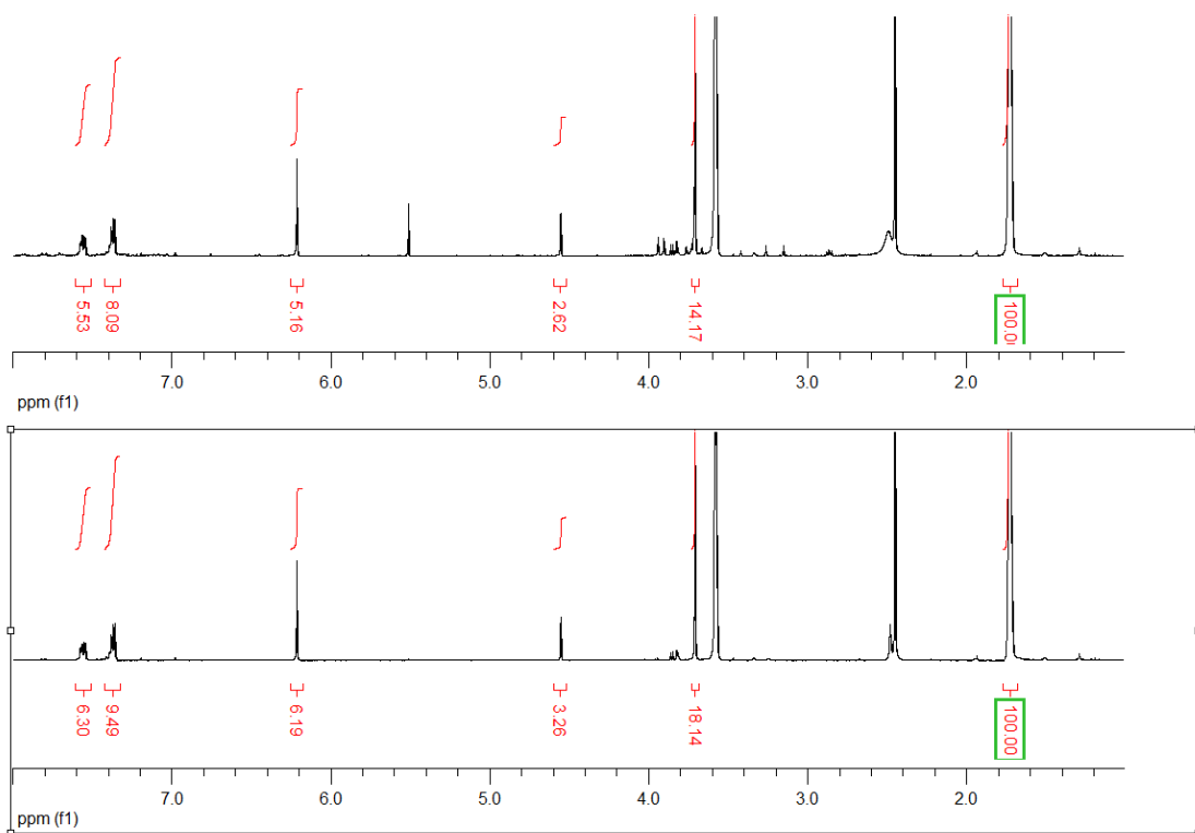
Figure S3. 1 H NMR spectra of BI 2 H in deuterated aerated THF over 20 hours. Stability estimated by arbitrarily pinning THF residual proton signal (1.73 ppm) at 100 integration. 83% of BI 1 H is estimated to remain after 20 hours in THF.
