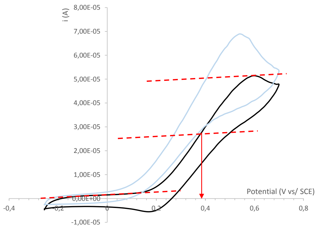
Figure S4. Cyclic voltamperometry of BI 1 H in THF (black line) and in presence of 1 equivalent of TEA (blue line) with glassy carbon as working electrode, platinum grid for counter electrode and SCE for the reference electrode.
