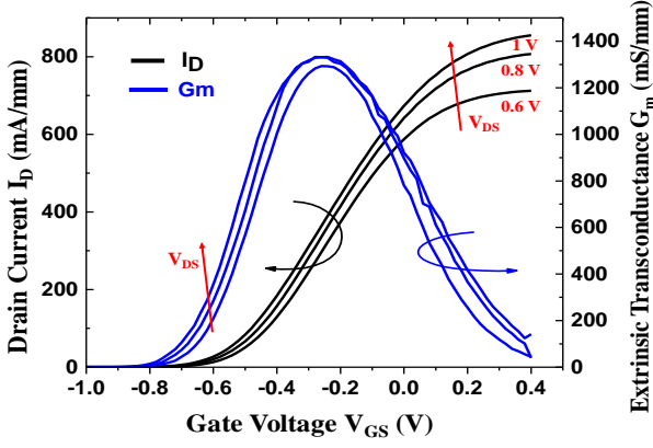
Fig. 4. Transfer and transconductance characteristics of the L_G = 75 nm and W_G = 2 \times 12 \mu\text{m} PHEMT.
