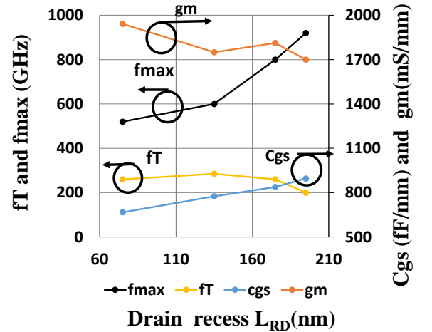
Fig. 7(b). Evolution of f_{\text{max}} , C_{gs} and g_m versus drain side recess L_{RD} . The source side recess L_{RS} is kept at 65 nm.
