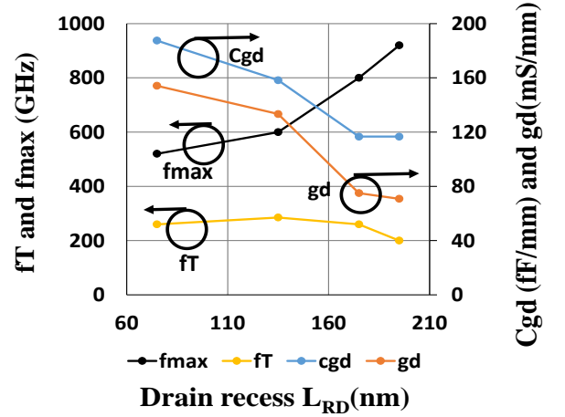
Fig. 7(a). Evolution of f_{\text{max}} , C_{gd} and g_d and versus drain side recess L_{RD} . The source side recess L_{RS} is kept at 65 nm.
