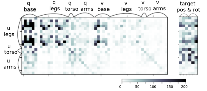
Fig. 2. Left: matrix of the absolute Riccati gain K_0 for a whole-body OCP involving end-effector tracking and biped stabilization. Right: matrix of the absolute placement (position and rotation) gains for a whole-body OCP involving tracking a reference placement with the left hand while stabilizing balance.
