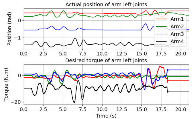
Fig. 6. Disturbance experiment: the MPC is shut down and external disturbances are manually applied.
