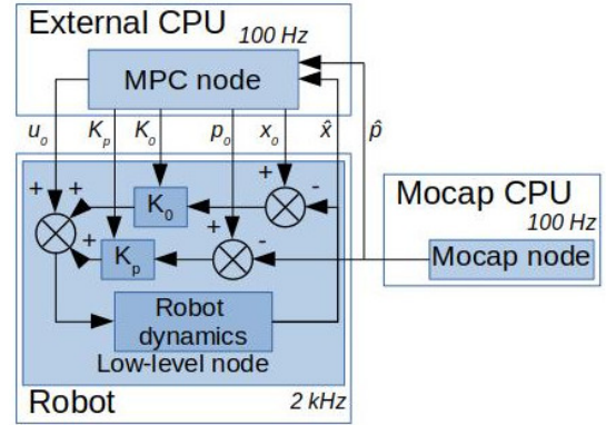
Fig. 3. Diagram of the ROS implementation of the Riccati feedback MPC.
