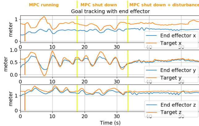
Fig. 8. Placement feedback experiment tracking plot.
