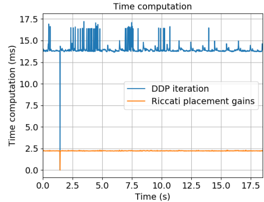
Fig. 9. Placement feedback experiment time plot.
