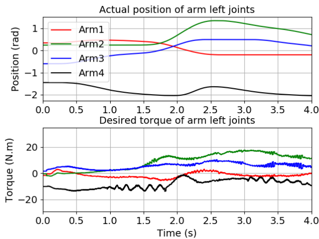
Fig. 5. Whole-body tracking experiment with Riccati gains. Although some oscillations remain, the overall tracking behaviour is good.
