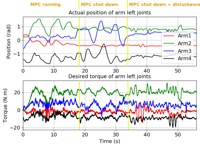
Fig. 7. Placement feedback experiment state and control plot: MPC is shut down at t = 18s , and external disturbances start to be applied at t = 33s .
