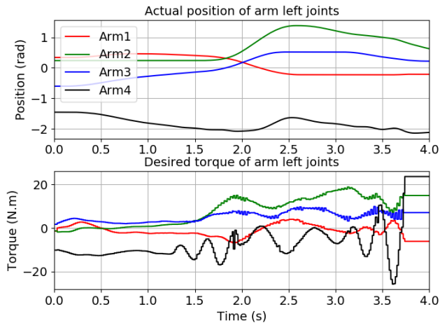
Fig. 4. Whole-body tracking experiment without Riccati gains. After 4 seconds, the desired torque oscillations become too large, and the securities of the robot are triggered, shutting down all motors.
