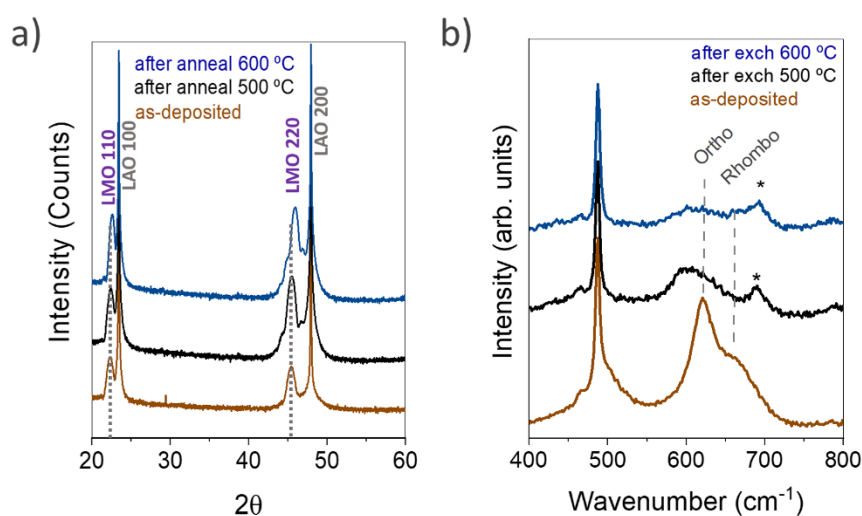
Fig. 5. a) XRD patterns obtained for the epitaxial LMO/LAO thin film as deposited and after anneals at 500 and 600 °C. LMO and LAO peaks indexed in the orthorhombic and pseudocubic systems, respectively. b) Raman spectra of the LMO/LAO thin films as deposited and after the exchanges at 500 and 600 °C. The positions of the orthorhombic and rhombohedral lines in the pristine spectrum are indicated by the grey dashed lines. The exact assignment of the peak * is not clear, and might correspond to the \text{Mn}_2\text{O}_3 or to the \text{LaMnO}_3 phase. The narrow line at 487\text{ cm}^{-1} is related to the LAO substrate. For both figures, the pattern in brown corresponds to the as-deposited (pristine) LMO film, the black one was obtained after annealing (exchange) at 500 °C and the blue one after annealing (exchange) at 600 °C.
