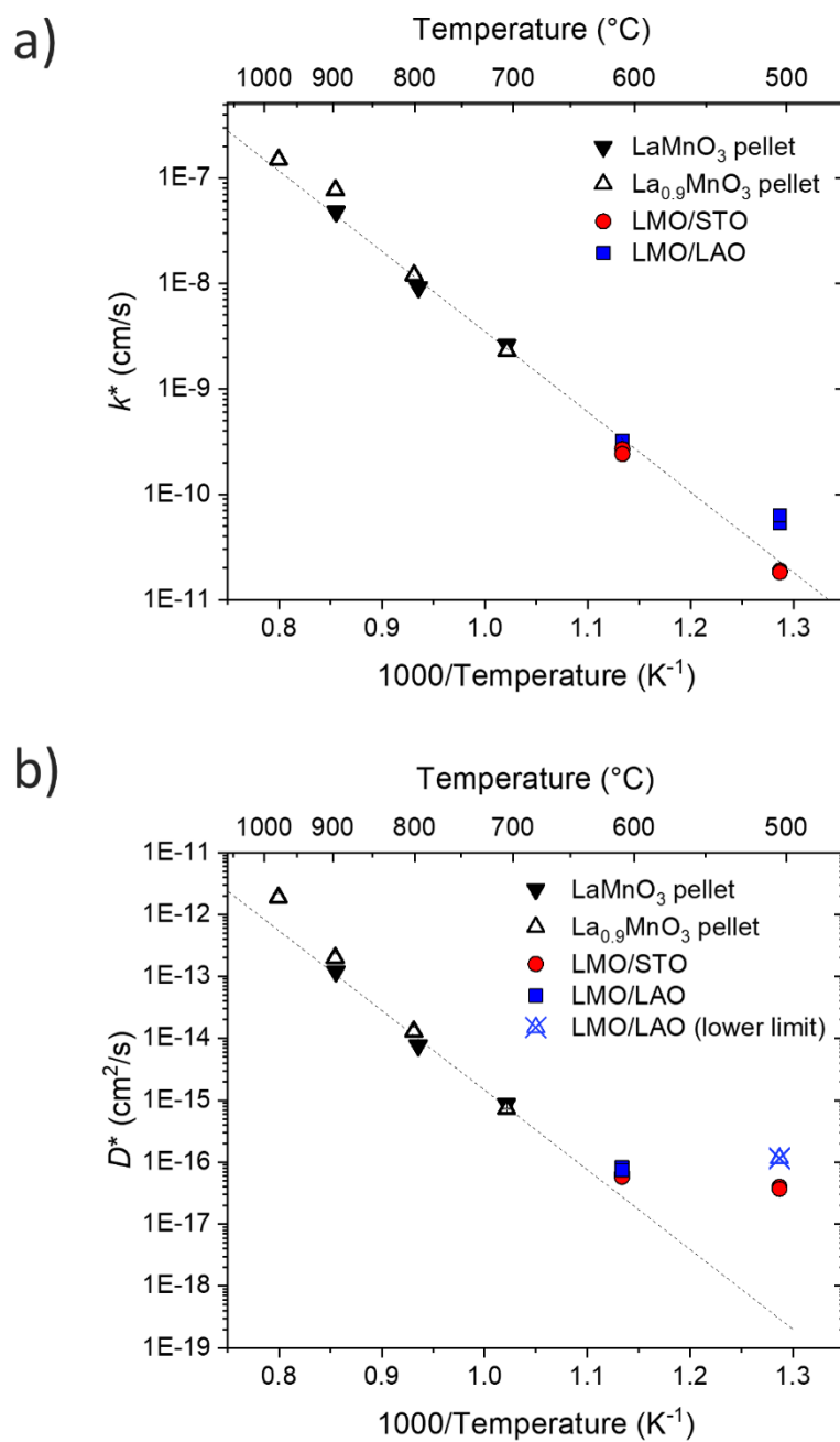
Fig. 3 Arrhenius plots of the oxygen tracer: a) surface exchange and b) diffusion coefficients for LMO/STO and LMO/LAO epitaxial films grown by PI-MOCVD (this work). Comparison with data obtained for LaMnO_3 and La_{0.9}MnO_3 pellets from Berenov et. al. 40 .
