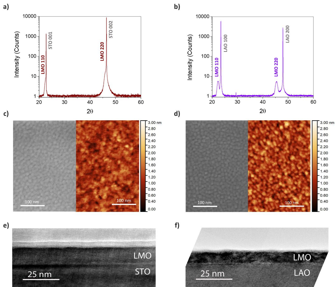
Fig. 1. Structural characterization of the dense thin LMO films. XRD \theta - 2\theta patterns obtained for as-deposited films: a) LMO/STO, b) LMO/LAO. LMO, LAO and STO peaks are indexed in the orthorhombic, pseudocubic and cubic systems, respectively. SEM (left) and AFM (right) top views including the AFM height scale (right), providing a topography image and a roughness reference of the films after the exchange at 500 °C: c) LMO/STO, d) LMO/LAO, respectively. TEM bright field cross-section image of the films exchanged at 500 °C: e) LMO/STO, ~12 nm thick, seen along the [001] zone axis for STO and f) LMO/LAO, ~11 nm thick, seen along the [001] zone axis for LAO.
