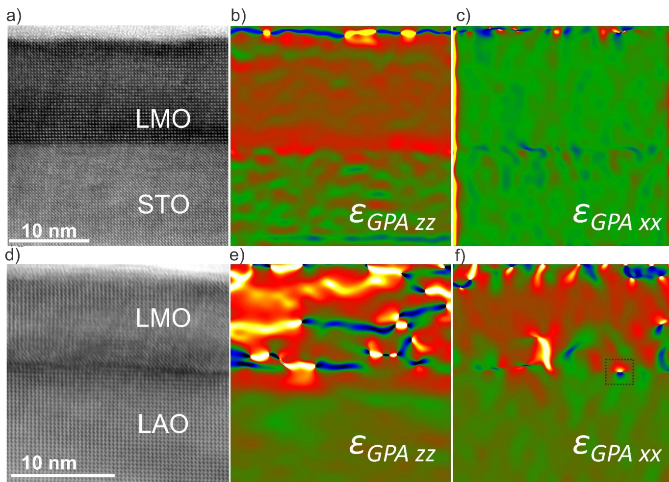
Fig. 5(a) HRTEM image of the 12 nm epitaxial LMO/STO film exchanged at 500°C seen along the STO [001] zone axis. (b) Corresponding GPA strain image ( \epsilon_{GPA\ zz} ) of the LMO layer with respect to the STO substrate along the [-1-10]_{LMO} // [100]_{STO} . The STO substrate is used as reference (i.e. \epsilon_{GPA\ zz} = 0\% ) while the average \epsilon_{GPA\ zz} in the LMO film is found equal to 2.3 \pm 1\% . (c) Corresponding GPA strain image ( \epsilon_{GPA\ xx} ) of the LMO layer with respect to the STO substrate along the [-110]_{LMO} // [010]_{STO} . A negligible \epsilon_{GPA\ xx} has been found. (d) HRTEM image of the 11 nm epitaxial LMO/LAO film exchanged at 500°C seen along the LAO [001] zone axis. (e) Corresponding GPA strain image ( \epsilon_{GPA\ zz} ) of the LMO layer with respect to the LAO substrate along the [-110]_{LMO} // [010]_{LAO} . The LAO substrate is used as reference (i.e. \epsilon_{GPA\ zz} = 0\% ). An average \epsilon_{GPA\ zz} in the LMO film is difficult to estimate due to the presence of a large number of extended defects. (f) Corresponding GPA strain image ( \epsilon_{GPA\ xx} ) of the LMO layer with respect to the LAO substrate along the [-1-10]_{LMO} // [010]_{LAO} . The LAO substrate is used as reference (i.e. \epsilon_{GPA\ xx} = 0\% ) while the average \epsilon_{GPA\ xx} in the LMO film is found equal to 2.5 \pm 1\% . The square denote the presence of a misfit dislocation in the LAO/LMO interface.
