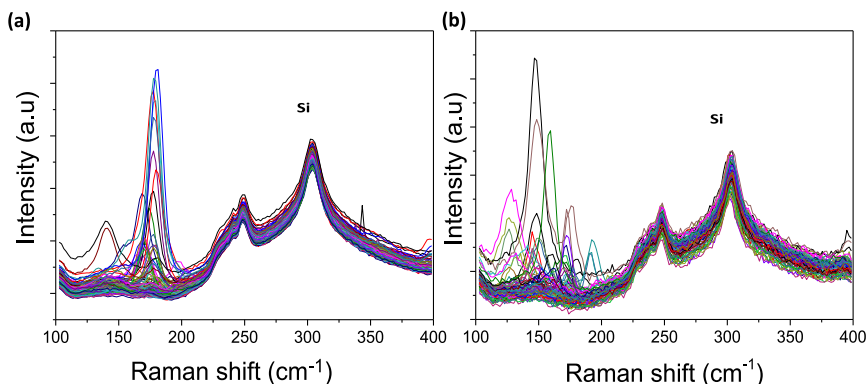
Fig. 1. (a) Raman radial breathing mode (RBM) spectra of SWNTs synthesized from a 0.05 nm-thick Ru layer at 850 °C under atomic hydrogen flux ( H_{at} ). (b) RBM spectra of SWNTs functionalized with Co-Po.
