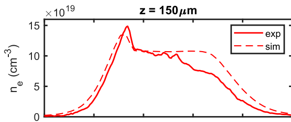
FIG. 6. Comparison of measured and simulated plasma profile obtained with a one-sided shock nozzle using nitrogen with a backing pressure of 15 bar at a distance of 150 \mu\text{m}
