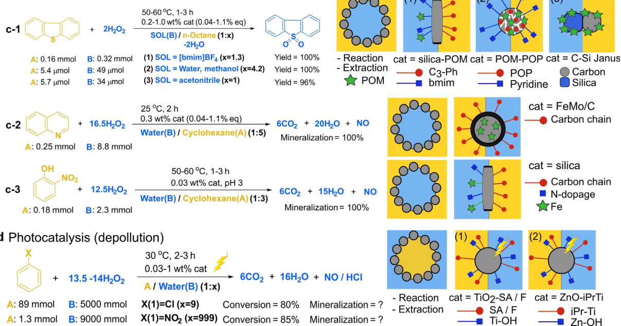
Figure 3. Particle-stabilized L-L-S microreactors for oxidation reactions: a) Epoxidation of olefins, [75,76,81] b) Partial oxidation of alcohols, [83,85,89] benzene hydroxylation, [90] and oxidation of sulfides [91] for synthesis; c) Partial/total oxidation [92-96] and photocatalytic oxidation [97,98] for depollution.
