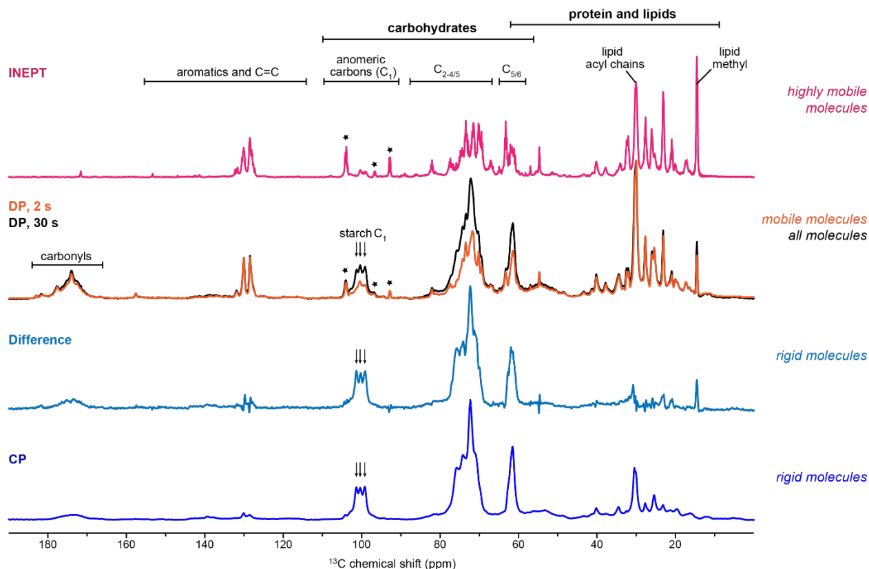
Figure 2. Dynamic heterogeneity of microalgal molecules revealed by 1D 13 C ssNMR spectra. The J -coupling-based refocused INEPT spectrum (magenta) only shows signals of highly mobile molecules. 13 C DP spectra with a long recycle delay (30 s; black) enables quantitative detection while a short recycle delay (2 s, orange) detects mobile components. Arrows and stars are respectively used to highlight the carbon 1 sites of rigid starch and C1 of mobile carbohydrates. The difference spectrum (light blue) of the two DP parental spectra is highly similar to the CP spectrum (blue), selecting rigid molecules. All spectra were collected using intact P. beijerinckii cells on an 800 MHz NMR spectrometer, with 13.5 kHz MAS frequency and 83 kHz TPPM 1 H decoupling.
