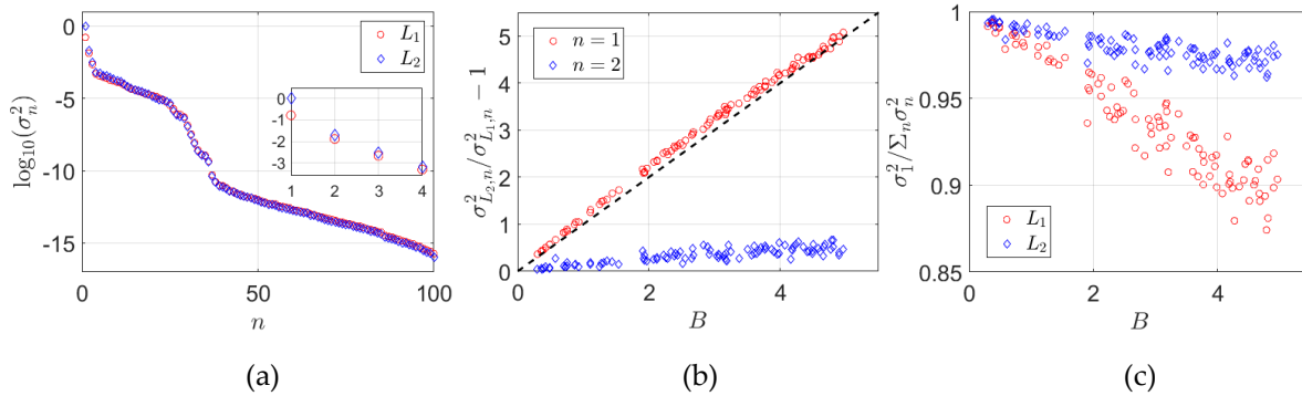
Figure 1. (a) PCA variance obtained with the two distinct weighting matrixes, \mathbf{L}_1 and \mathbf{L}_2 . The results are normalized by \sigma_1^2 obtained with \mathbf{L}_2 . (b) Ratio of the PCA variances obtained with the two weights as a function of B , for the first and second principal components. (c) Ratio of the first PCA variance to the total variance as a function of B , for \mathbf{L}_1 and \mathbf{L}_2 .
