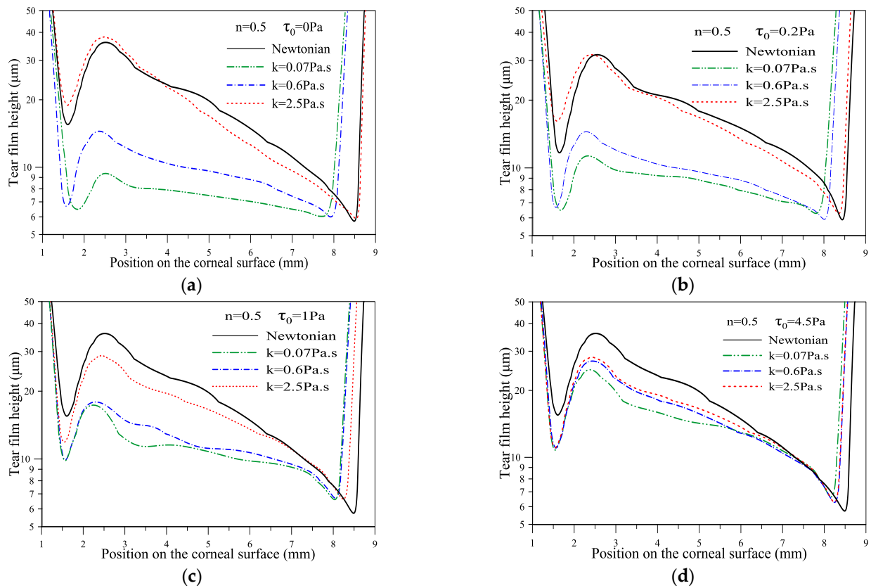
Figure 4. (a–d) the effect of consistency k , n = 0.5 , \tau_0 = 0, 0.2, 1 and 4.5 Pa at t = 0.18 s.
