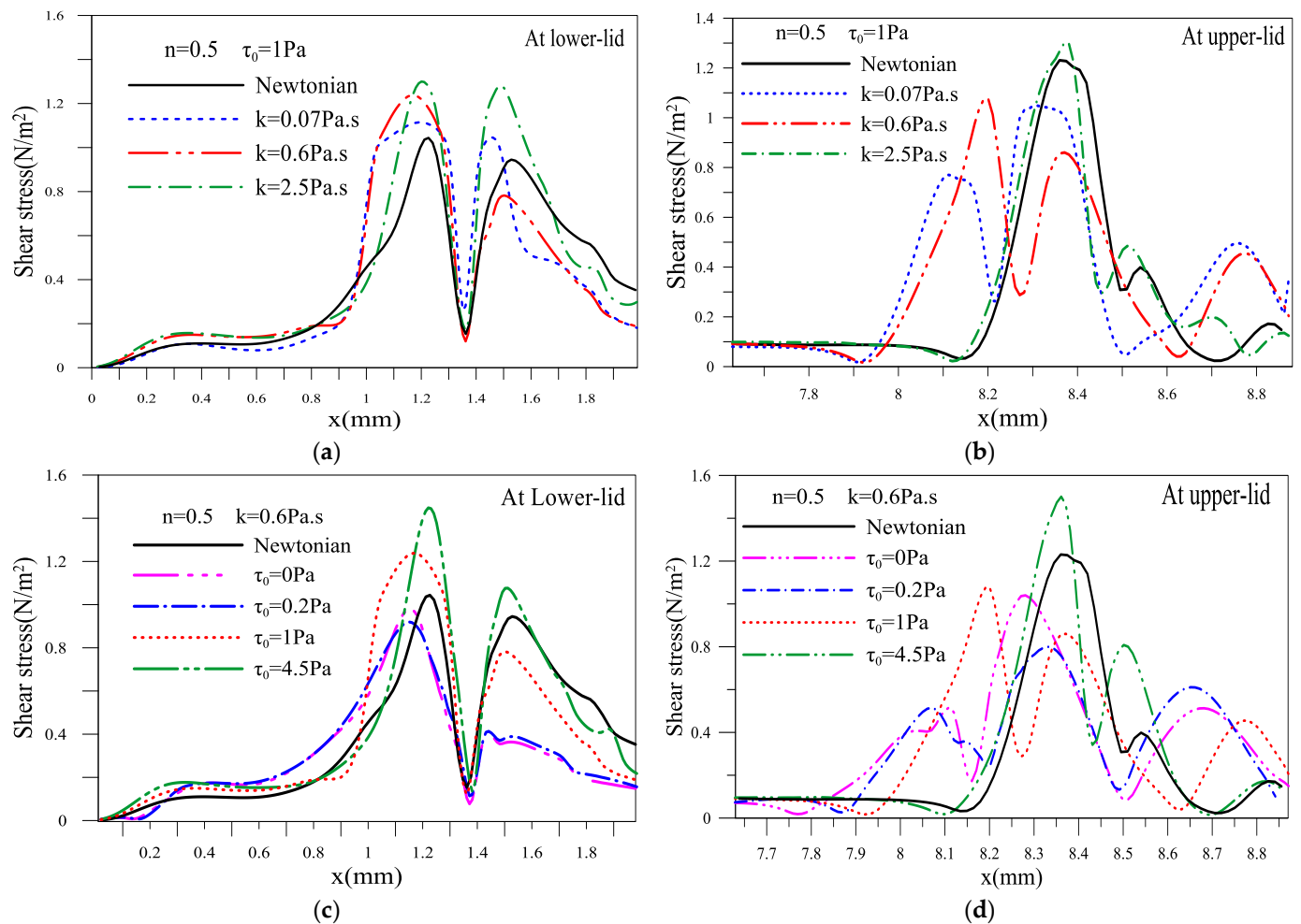
Figure 8. Variation of wall shear stress: (a,b) consistency k effect; (c,d) yield stress \tau_0 effect.
