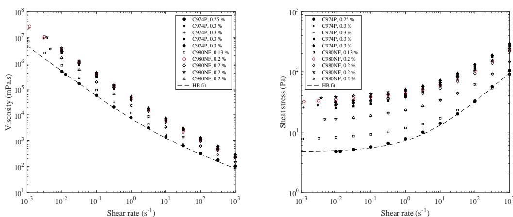
Figure 1. Flow curves of gel tears at 25 °C: yield stress and very high viscosity at a low shear rate and decreasing viscosity during a blink (high shear rate). The grey lines represent the Hershel-Bulkley model applied to the product with the lowest yield stress.
