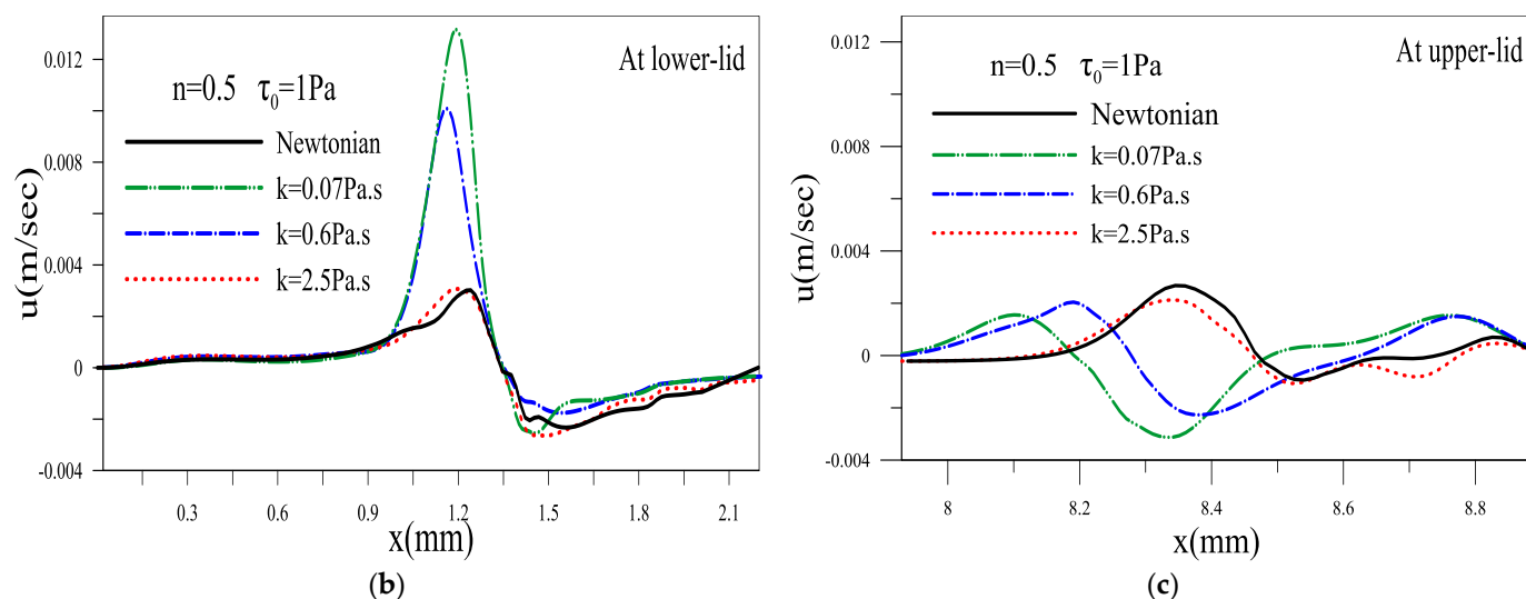
Figure 6. Depth average velocity for different consistency k , at time = 0.18 s. (a) over the whole cornea surface (b) and (c) a closeup near the lower and upper eyelid.
