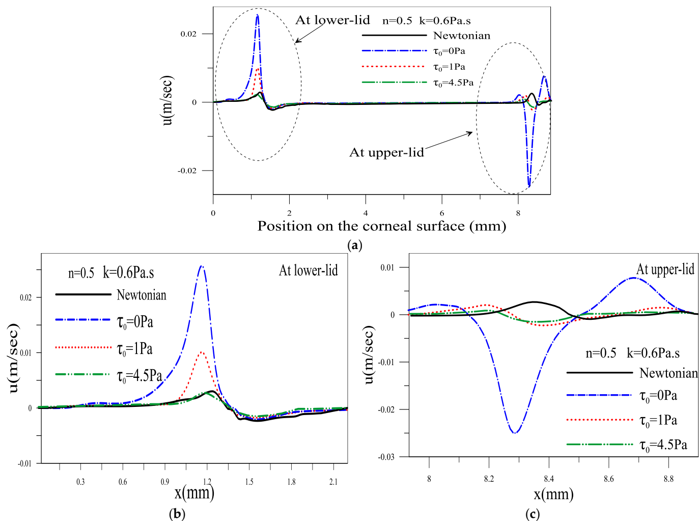
Figure 7. Depth average velocity for different yield stress ( \tau_0 ) at time = 0.18 s. (a) over the whole cornea surface, (b) and (c) a closeup near the lower and upper eyelid.
