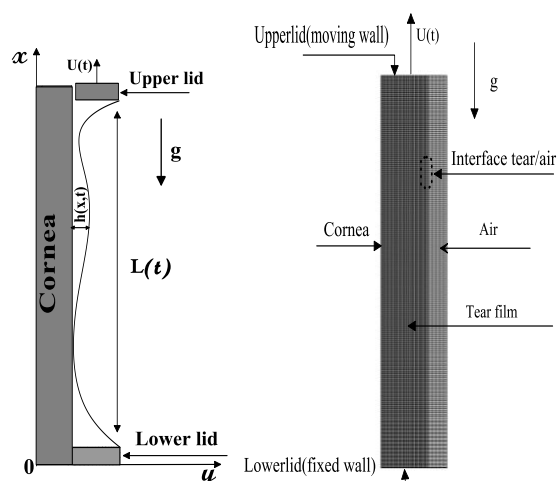
Figure 9. Physical and numerical domain of the tear film problem.
