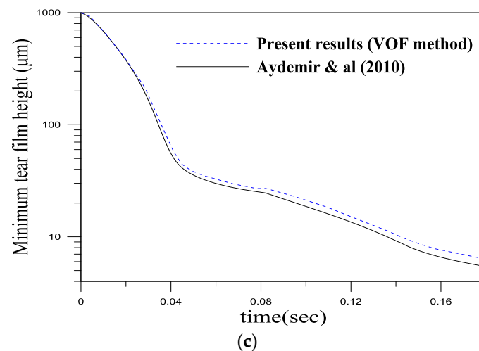
Figure 11. Model validation against the model by Aydemir's work [25]. (a,b) film thickness distribution along the planar substrate at 0.04 and 0.18 sec, respectively. (c) Evolution of the minimum tear film thickness with time. The parameters of the simulations are: \rho = 10^{-3} \text{ kg}\cdot\text{m}^{-3} , \mu = 1.3 \times 10^{-3} \text{ Pa}\cdot\text{s} , \sigma = 0.045 \text{ N/m} , h^* = 0.001 \text{ m} , L_{cl} = 0.002 \text{ m} , L_{op} = 0.01 \text{ m} , U_0 = 0.0163 \text{ m/s} .
