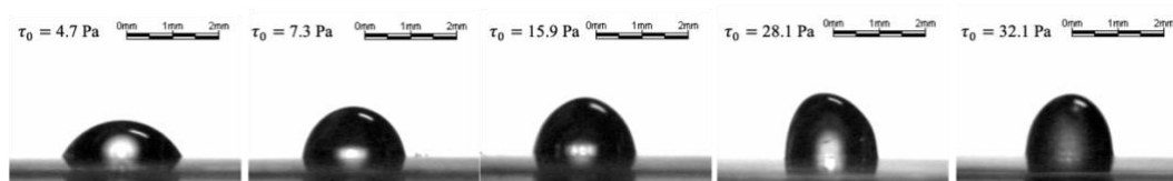
Figure 2. Spreading of gel tears with various yield stresses.
