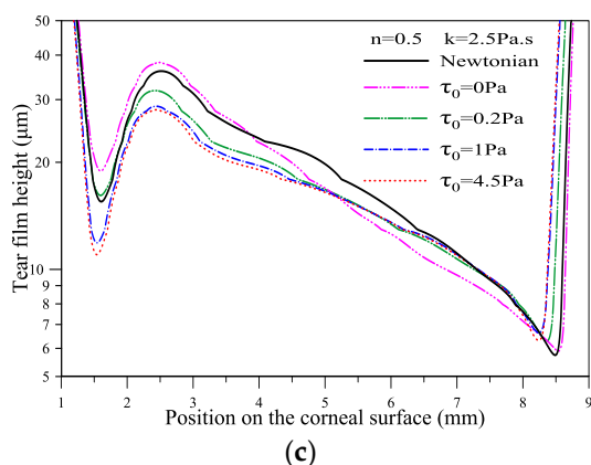
Figure 5. Variation of film thickness for different \tau_0 , n = 0.5 at t = 0.18 s. a) k = 0.07 , b) k = 0.6 , c) k = 2.5 Pa·s.
