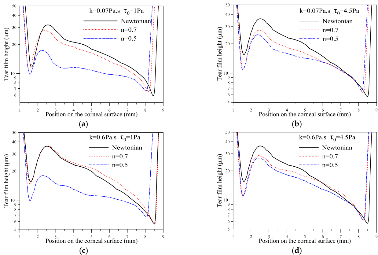
Figure 3. Effect of flow index, n , on variation of film thickness for \tau_0 = 1 and 4.5 \text{ Pa} , k = 0.07 and 0.6 \text{ Pa}\cdot\text{s} at t = 0.18 \text{ s} . Q = 10^3 \text{ kg}\cdot\text{m}^{-1} , \mu = 1.3 \times 10^{-3} \text{ Pa}\cdot\text{s} (Newtonian case), \sigma = 0.045 \text{ N/m} , h^* = 0.0005 \text{ m} , L_{cl} = 0.001 \text{ m} , L_{op} = 0.01 \text{ m} , U_0 = 0.0163 \text{ m/s} .
