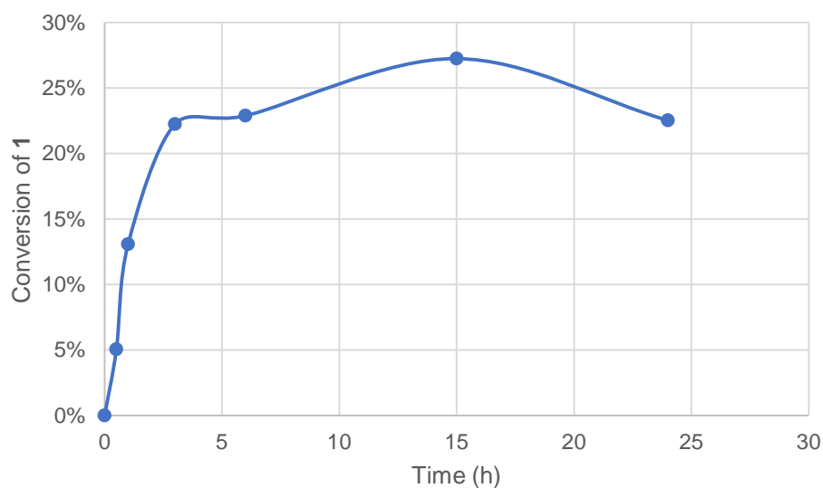
240 241 Figure 6. Effect of time reaction on conversion of 1 in the laccase-catalyzed oxidation (LA 10% w/w , 242 HOBT 20 mol%, acetate buffer pH5 0.25 M, O 2 atmosphere, incubation 40 °C, 200 rpm).
