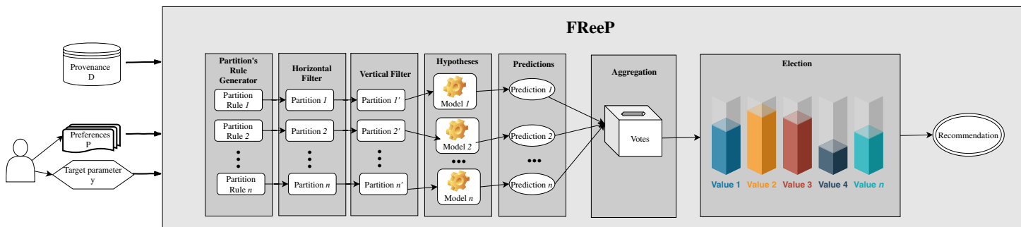
Figure 4 FFreeP architecture overview.
