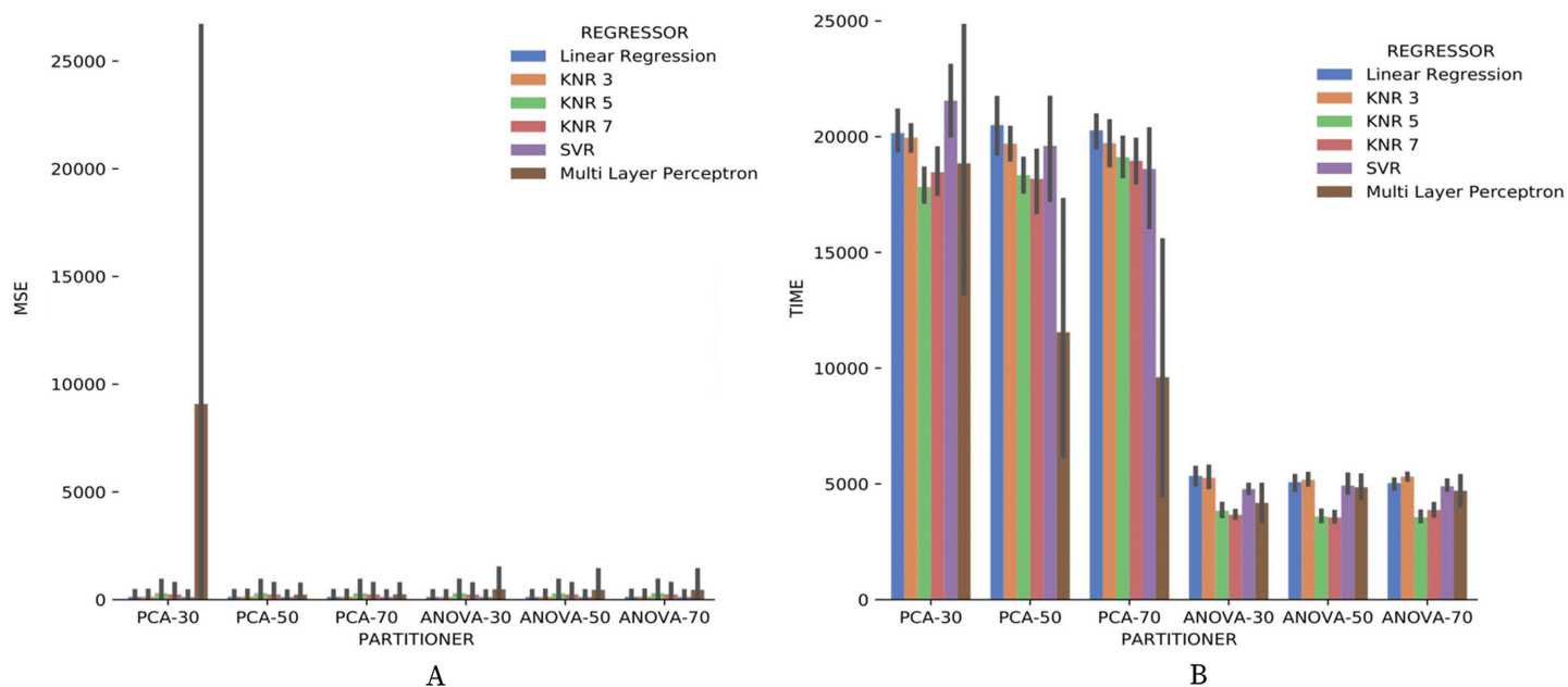
Figure 24 MSE results and recommendation execution time with Montage data.
