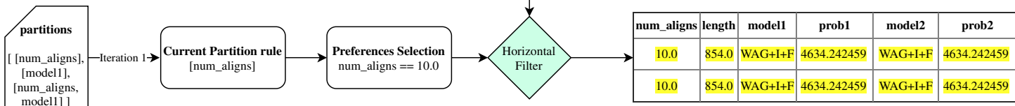
Figure 6 Example of FReeP 's horizontal filter using one partitioning rule for the Sciphy provenance dataset.
