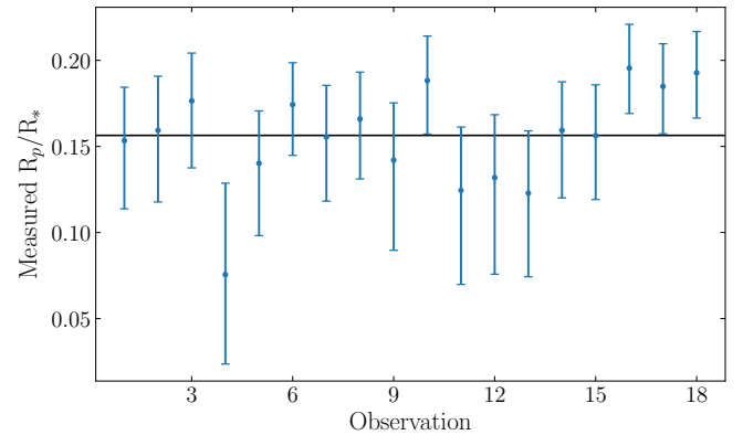
Figure 2. Measured value of the ratio of the planet and stellar radius, R_{p,UVW2}/R_* , in each transit observation with the UVW2 filter on the Optical Monitor. The solid horizontal line depicts the measured value of R_p/R_* at optical wavelengths.
