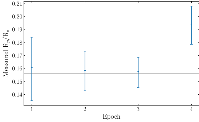
Figure 3. Measured value of the ratio of the planet and stellar radius, R_{p,UVW2}/R_* , at each of the four defined epochs (see main text). The solid horizontal line depicts the measured value of R_p/R_* at optical wavelengths.
