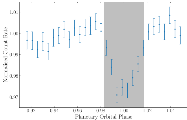
Figure 1. Binned, phase folded OM light curve for the 18 observations with UVW2. No correction has been made in this figure for out of transit trends. The shaded region is the full duration of the optical transit, with the phases plotted according to the ephemeris in Table 1.
