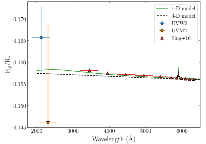
Figure 7. Transmission spectrum of HD 189733b in the optical and NUV. The points associated with the transit measurements presented in this work are given with the blue circle (UVW2 filter), and orange star (UVM2). The red triangles are the data presented in Sing et al. (2016) (only that blueward of 6500 Å is displayed) - the errorbars on those points are too small to be seen on this scale. The green solid line is that expected by the 1-D model extended from the work of Lavvas & Arfaux (2021), and the black dashed line is that expected by the 3-D model extended from the work of Steinrueck et al. (2020). The Roche lobe of the planet ( 3 R_{opt} , or R_p/R_* = 0.471 ) is too far off the scale of the plot to be visible.
