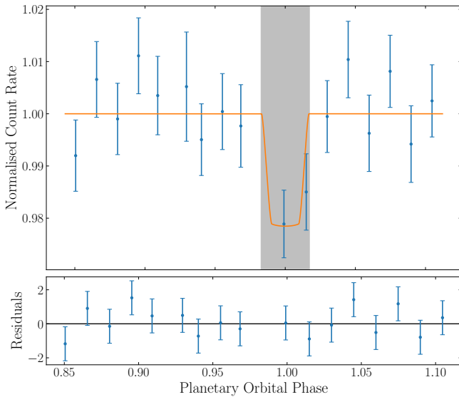
Figure 6. As Fig. 4, but for the single UVM2 light curve and associated fit.
