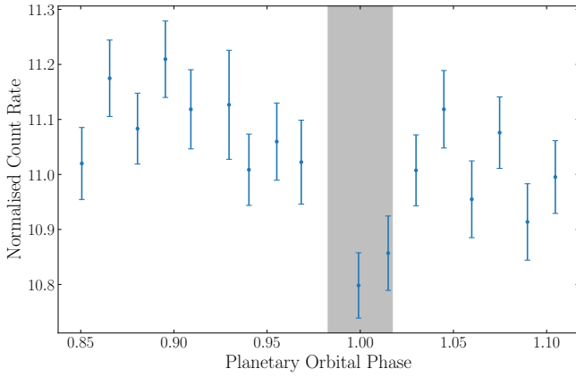
Figure 5. Binned OM UVM2 light curve for observation 1. This time series has not been corrected for out of transit trends.
