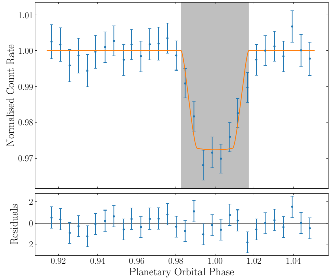
Figure 4. Top panel: binned, phase folded OM light curve for the 18 UVW2 observations, with the best fitting out of transit quadratic trends removed. Plotted in orange is the best fit model, where R_{p,UVW2} was forced to be constant across all 18 light curves. Bottom panel: residuals of the model.
