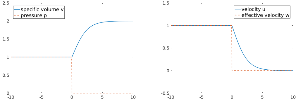
Figure 1: On the left: the profiles \bar{v} and \bar{p} , on the right: the profiles \bar{u} and \bar{w} .
