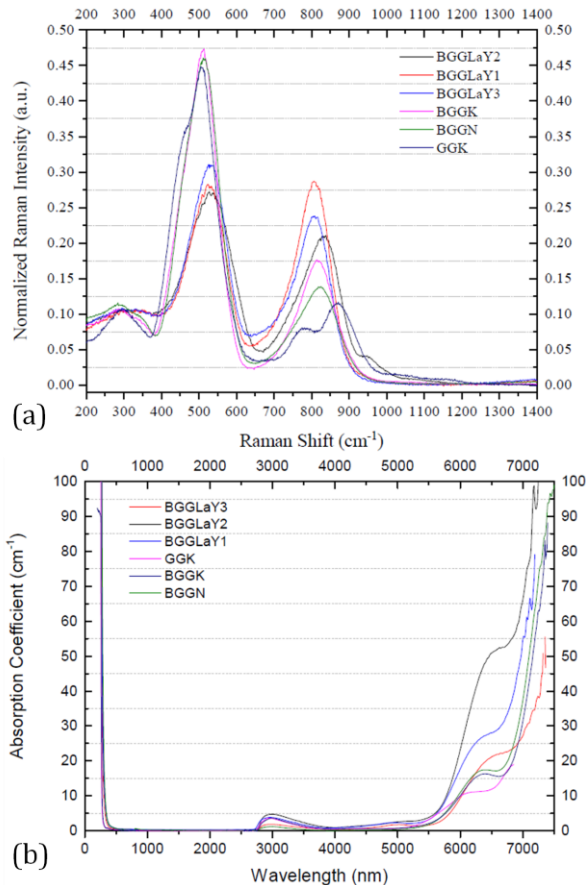
Fig. 1. (a) Normalized Raman Intensity of GGK, BGGLaY1, BGGLaY2, BGGLaY3, BGGK and BGGN glasses as a function of Raman shift. (b) Absorption coefficients of GGK, BGGLaY1, BGGLaY2, BGGLaY3, BGGK and BGGN glasses as a function of wavelength.
