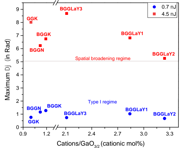
Fig. 4. Maximum phase shift ( \Delta\phi , in Rad) as a function of Cations/GaO 3/2 (in cationic mol%).
