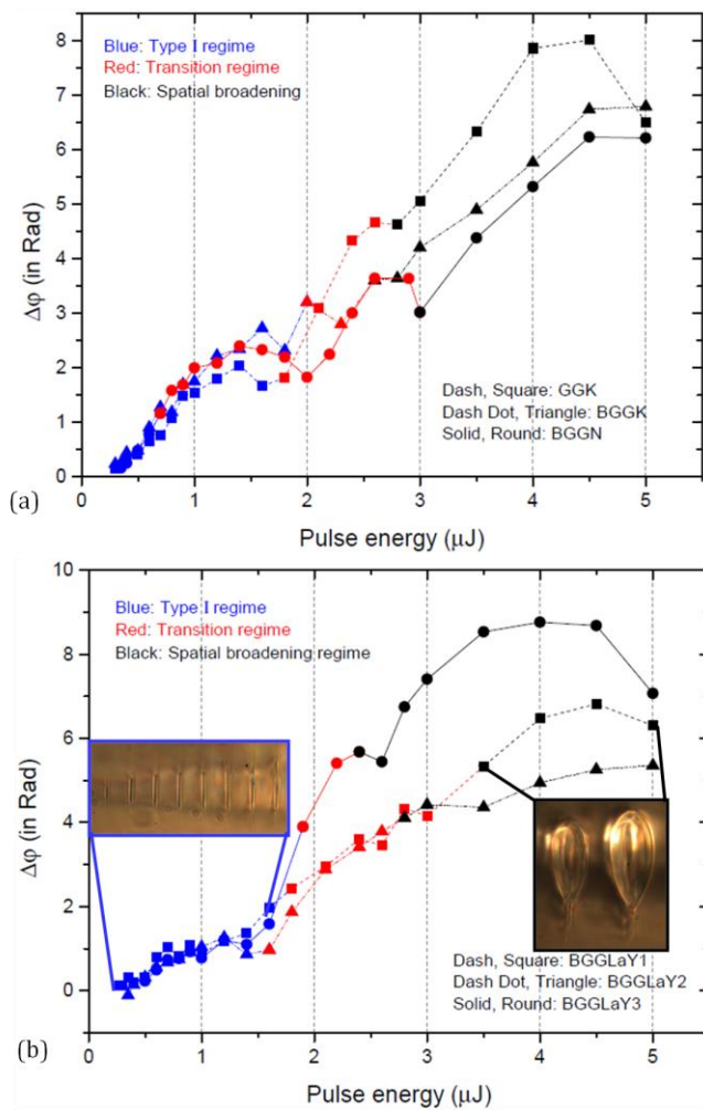
Fig. 3. (a) Phase shift (in rad) for GGK, BGGK and BGGN glasses as a function of pulse energy. (b) Phase shift for BGGLaY1, BGGLaY2 and BGGLaY3 glasses. Left inset: optical image of BGGLaY1 in low energy. Right inset: optical image of BGGLaY1 (3 \mu J and 2.5 \mu J from left to right). Lines are guide-to-the-eye.
