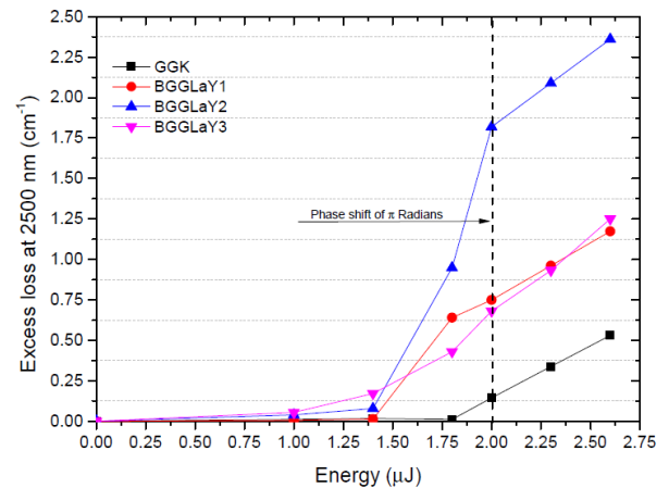
Fig. 5. Excess loss at 2500 nm as a function of energy for GGK, BGGLaY1, BGGLaY2 and BGGLaY3 glasses after fs laser irradiation.
