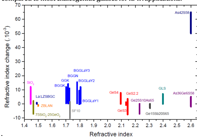
Fig. 6. Ranges of refractive index variations vs. refractive index (typ. measured at 532 nm) for the BGG, chalcogenide, fluoride, \text{SiO}_2 and germanate glasses.
