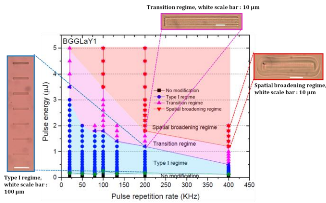
Fig. 2. Pulse energy – repetition rate landscape and identification of Type I regime, transition regime and spatial broadening regime in BGGLaY1 glass.
