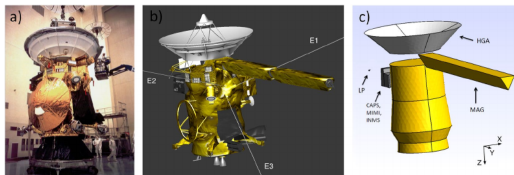
Figure 1. (a) The Cassini spacecraft prior to launch (image credit NASA/JPL-Caltech). (b) The detailed 3D model of Cassini, including the Radio and Plasma Wave Science (RPWS) electric field antennas, marked E1 to E3. (c) The simplified Cassini spacecraft model suitable for Spacecraft Plasma Interaction Software (SPIS) simulations. Panel (a) also shows the Huygens probe, the large golden dish attached to the side of the spacecraft, which was released soon after the orbit insertion and therefore excluded from the SPIS model.
