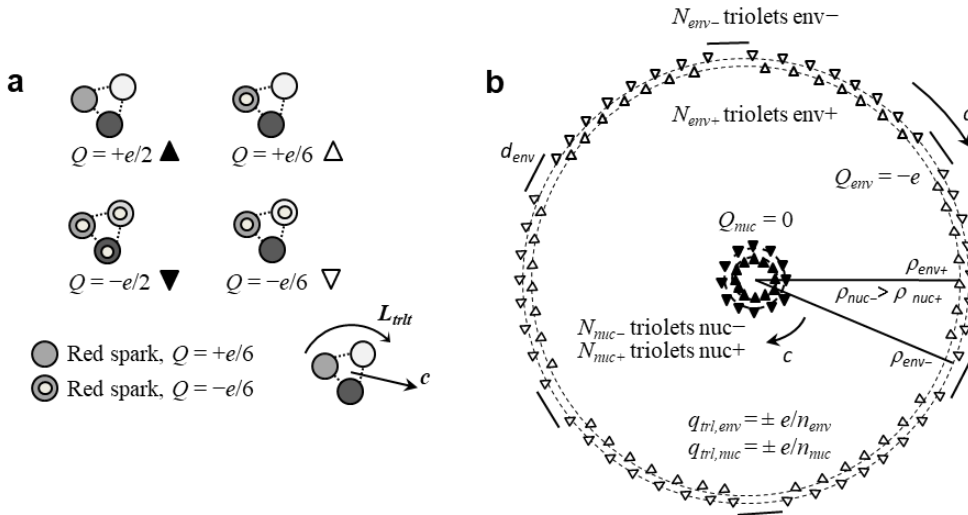
Fig. 2. a. Colorless triolets made of three colored ( \pm e/6 ) sparks exhibit four different electric charges, represented by filled or hollow upward or downward triangles. b. The granular model of the electron at rest presents triolets revolving at light velocity and constituting an envelope and nucleus.
