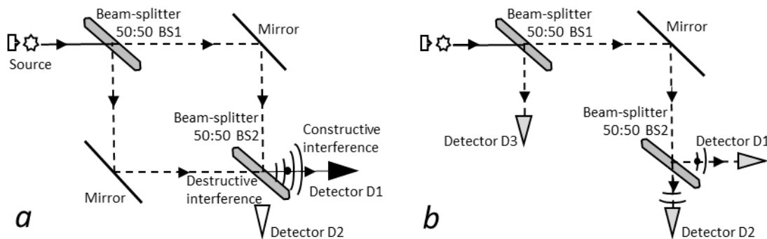
Fig. 1. Mach-Zehnder interferometer experiment. (a) Interference occurring at beam-splitter BS2 causes particles to be detected only at detector D1. (b) Particles undetected by detector D3 do not undergo interference at BS2 and are detected by both detectors D1 and D2.
