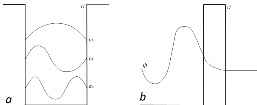
Fig. 3. a. Eigenstates in one-dimensional potential well. b. Tunneling.
