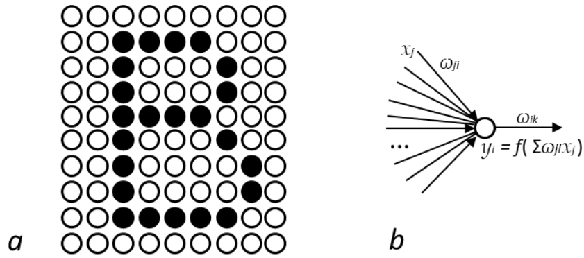
Fig. 4. a. Pattern (attractor) memorized in a recurrent neural network. b. Each neuron receives the weighted signal from all other neurons and emits a signal accordingly.
