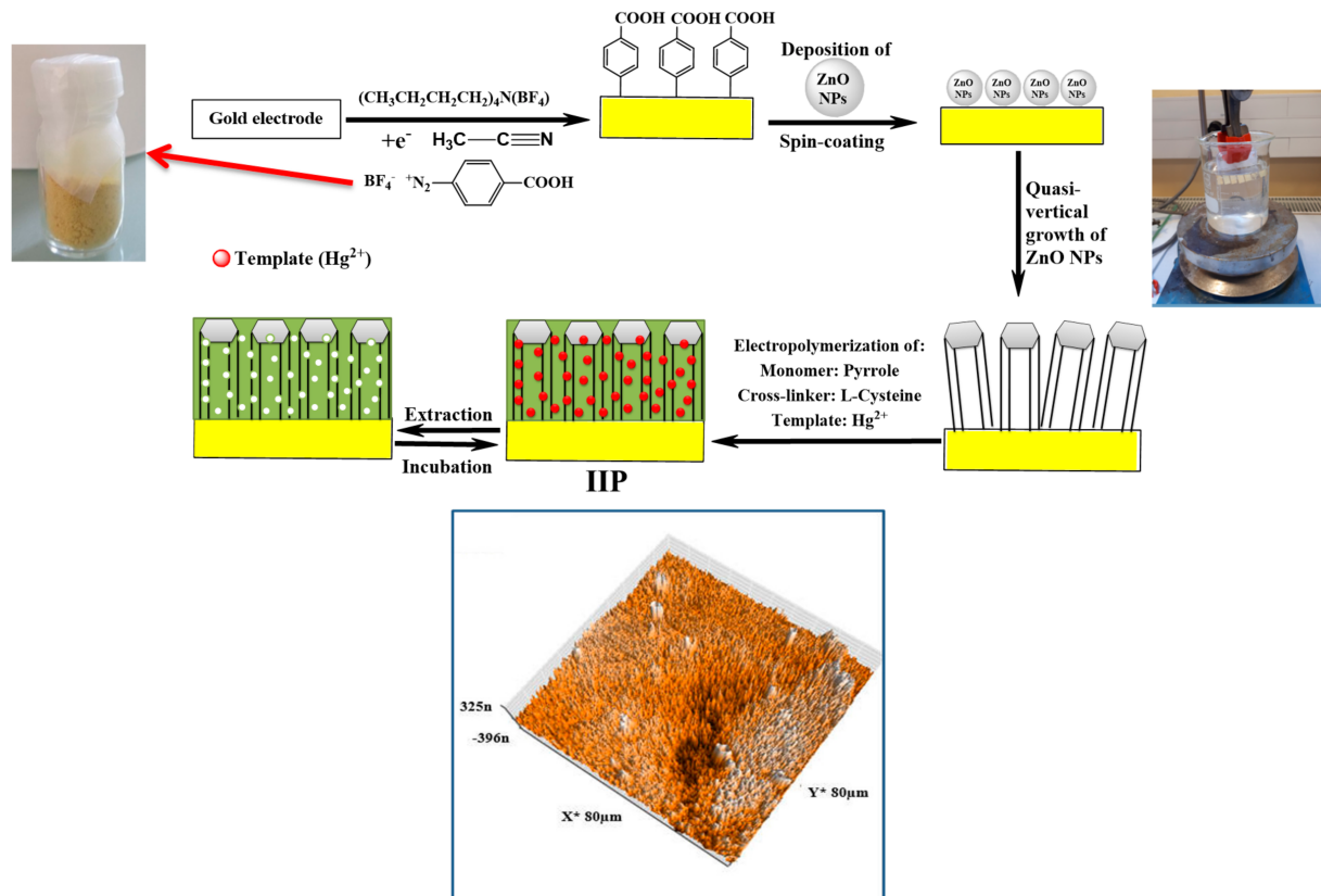
Figure 16. Top: Schematic illustration of the stepwise synthesis of mercury imprinted PPy wrapped around vertically aligned ZnO nanorods attached to diazonium-modified gold electrodes. Bottom: (80 \times 80 \mu\text{m}^2) 3D image of Au-diazo-ZnO NRs. Reproduced from [14].
