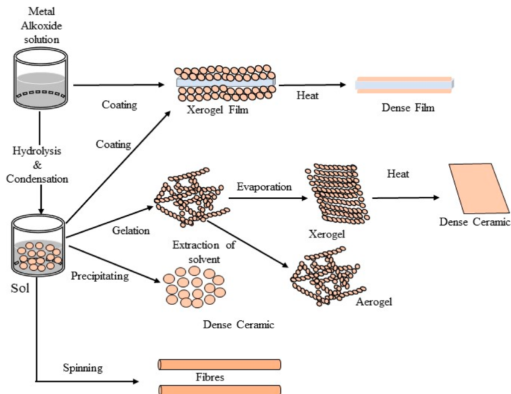
Figure 5. Sol-gel methods for nanoparticle synthesis.
