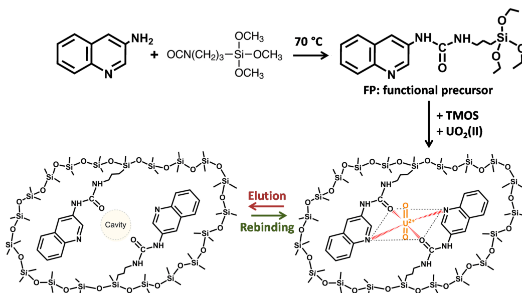
Figure 19. Synthesis of IISG from quinolone-functionalized silane, TMOS and uranyl. Adapted with permission of Elsevier from [130].
