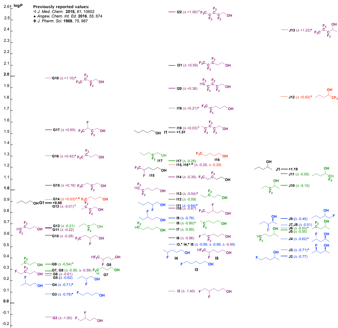
Figure 3. Summary table with new logP data, together with previously reported values for completion. 31,38,42 Color coding: blue, monofluorinated; green, gem -difluorinated; red, a (single) CF 3 group; purple, multifluorinated (fluorination at more than one carbon atom). The difference in logP value with the corresponding nonfluorinated parent compounds G1 , I1 , J1 (depicted in black) is given (See Figure S1 for a list of all logP values).
