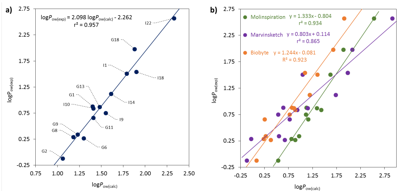
Figure 14. a) Correlation between the \log P_{\text{theor}} values, calculated after obtaining the (weighted) solvation energies in octanol and water, with the experimental \log P data for a subset of fluorohydrins. b) Correlation between the \text{Clog}P values obtained with three web-based calculators, with the experimental \log P values for the same fluorohydrin subset.
