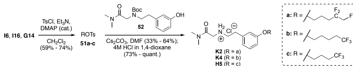
Scheme 6. Synthesis of evenamide analogues.
