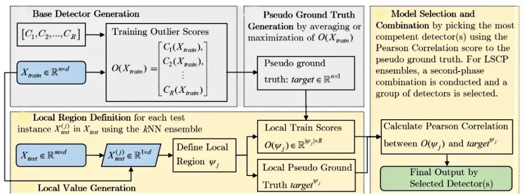
Figure 8. LSCP flowchart. Steps requiring recomputation highlighted in yellow; cached steps in grey [17].
