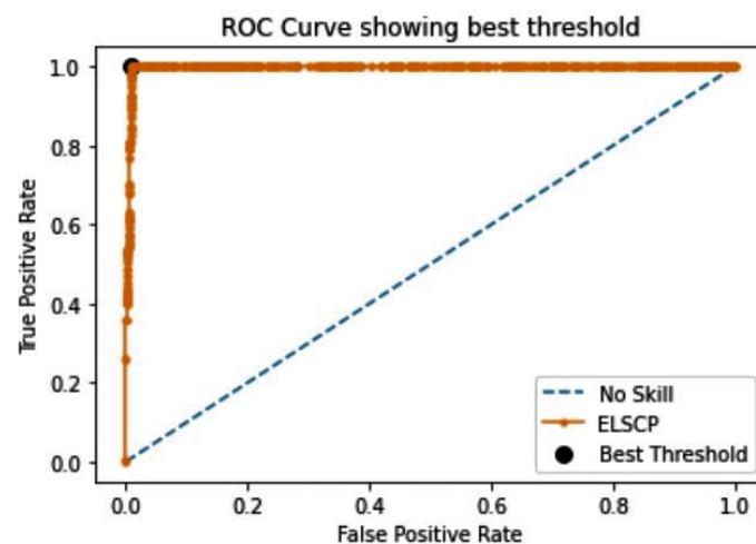
Figure 9. ELSCP ROC curve performance evaluation for combine-harvester GPS dataset.
