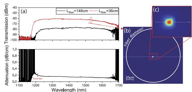
FIG. 2. (a)–(c) Transmission and modal properties of the silicon-core fiber. Left: optical transmission spectra for two different fiber lengths and attenuation curve deduced from those measurements. Right: near field image of the fiber output around 1500 nm wavelength with an imaging system permitting either a view of the whole fiber face or a zoom of the core region (inset).
