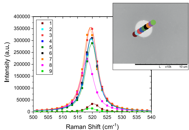
FIG. 3. Raman spectra recorded along a diameter of the 3.3\ \mu\text{m} -core fiber. In the inset, the position of the laser spots is superimposed on a SEM image of the fiber.
