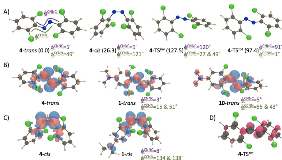
Figure 3. A) Representation of the DFT optimal geometries for the two stable isomers as well as inversion and rotation transition states, together with relative free energies in parenthesis (in \text{kJ mol}^{-1} ) and key dihedral angles for 4 ; B) electron density difference plot for the lowest transitions in three selected trans compounds. The blue and red lobes indicate regions of decrease and increase of density upon excitation, respectively. Representation threshold 15 \times 10^{-4} au; C) same for the cis isomers; D) spin density difference for the rotation transition state of 4 as given by BS-DFT. Representation threshold 10 \times 10^{-3} au.
