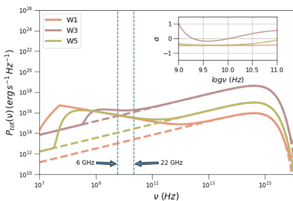
Figure 3. Radio-to-UV spectrum for three wind models and L_X = 10^{37} \text{ erg s}^{-1} . Left- and right-hand panels show results for \gamma_{\min} = 10 and 100, respectively. Thick solid and dashed lines show the total emission and thermal wind emission, respectively. Vertical dashed lines indicate two characteristic radio frequencies. In a strong wind scenario, like W3, the 6 GHz emission is dominated by the Be stellar wind. Inset plots show \alpha \equiv \text{dlog } P_{\text{tot}}(\nu)/\text{dlog } \nu as a function of frequency between 1 and 100 GHz.
