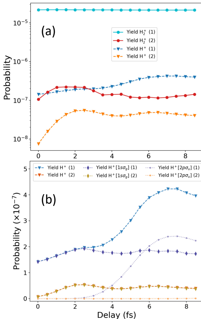
Fig. 9 Total ionization yields as a function of the time delay between the APT and the probe pulse for the scheme with the unfiltered pulse (scheme 1, blue lines labeled in the legends as [1]) and the scheme using the APT with the frequency filter (scheme 2, warm-coloured lines labeled in the legends as [2]). (a) Total non-dissociative ( H_2^+ ) and dissociative ( H+H^+ ) ionization signal for each scheme. (b) Total dissociative ionization yields ( H+H^+ ) are plotted again for each scheme in linear scale, together with the contributions from each cationic state.
