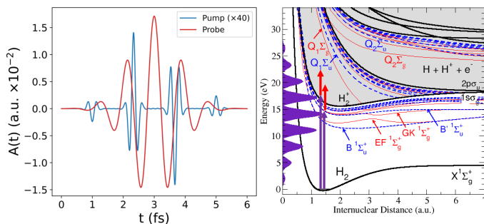
Fig. 1 (a) Vector potential, A(t) , for the attosecond pulse train (APT, in blue) and the 3rd harmonic (red) of a 800-nm IR field. Both pulses are defined with a total duration of 6 fs and intensities of 1.14 \times 10^9 and 3.0 \times 10^{11} W/cm 2 , respectively. (b) Energetics and relevant potential energy curves for the hydrogen molecule (see main text for details).
