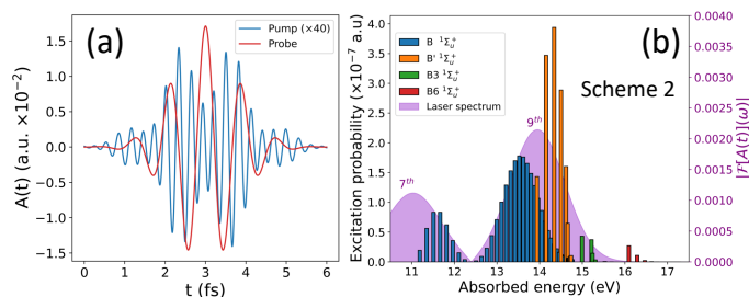
Fig. 5 (a) Vector potential A(t) for an attosecond pulse train after applying a frequency filter (blue), and the probe pulse with a frequency of the 3rd harmonic of the generating 800 nm IR field (red). (b) Excitation probabilities for the 1\Sigma_u^+ electronic states for the filtered pulse.
