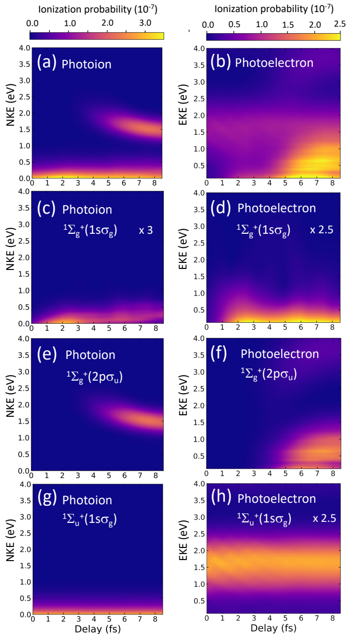
Fig. 3 Dissociative ionization yields ( \text{H}+\text{H}^++\text{e}^- ) as a function of the time-delay between pulses (x-axis) and of the kinetic energy of the charged fragments. Left panels: Photoion spectra. Right side panels: Photoelectron spectra. (a) and (b): total dissociative ionization yields as a function of the kinetic energy of nuclei and electrons, respectively. (c) and (d): two-photon dissociative ionization for the 1s\sigma_g state as a function of nuclear and electronic kinetic energies. (e) and (f): two-photon dissociative ionization for the 2p\sigma_u state of the ion. (g) and (h): dissociative ionization for an odd number of absorbed photons.
