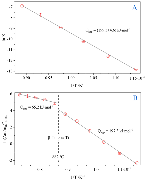
Fig. 10. (A) Arrhenius presentation of the parabolic proportionality constant K for synthesis temperatures up to 850°C; (B) Arrhenius presentation of the mass uptake after 10 h showing two kinetic regimes which appear to change at the \alpha \rightarrow \beta transition temperature.
