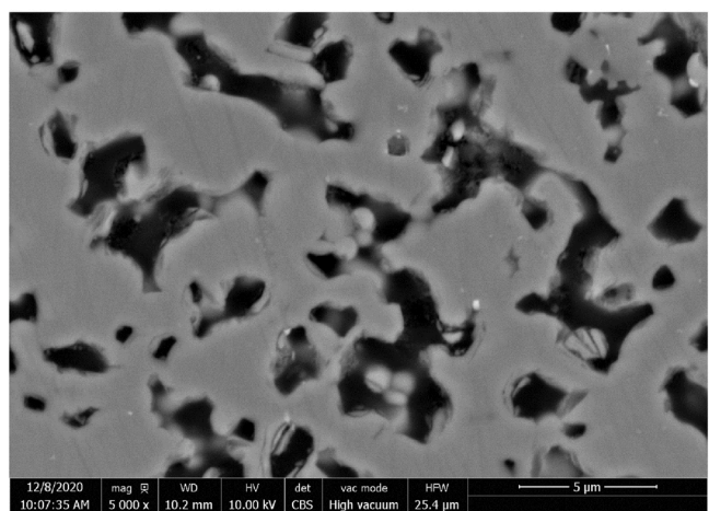
Fig. 12. SEM fracture micrographs of the SPS-smSiC sample after polishing. The final temperature was stopped at 1600 °C to avoid a full densification.
