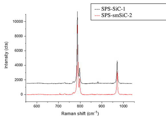
Fig. 7. Raman pattern of SPS-SiC-1 and SPS-smSiC-2.
