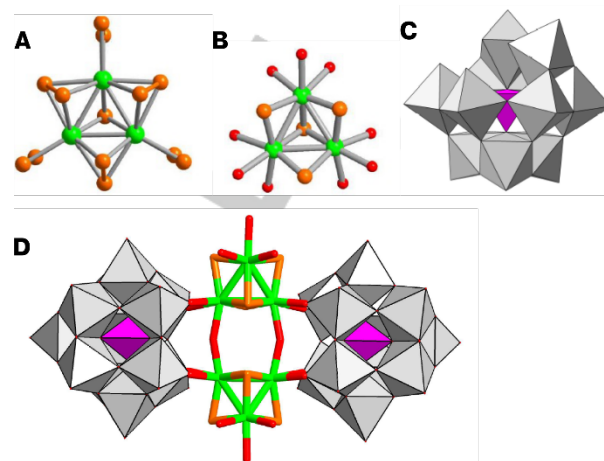
Figure 1 Structural representations of: (A) [Mo 3 S 13 ] 2- , (B) [Mo 3 S 4 (H 2 O) 9 ] 4+ , (C) [PW 11 O 39 ] 7- and (D) [((PW 11 O 39 )Mo 3 S 4 (H 2 O) 3 (μ-OH)) 2 ] 8- (Chalco-POM). Structural representation of the thio-POM resulting from the combination between [Mo 3 S 4 (H 2 O) 9 ] 4+ and α-A-[PW 11 O 39 ] 7- ions was derived from the reported structure of [((SiW 11 O 39 )Mo 3 S 4 (H 2 O) 3 (μ-OH)) 2 ] 10- cluster species (see ref 16).
