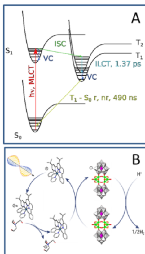
Figure 9. A) Proposed hypothesis of the excited state dynamics of [\text{Ir}] in \text{CH}_3\text{CN}/\text{DMF} (1/3), based on femto- and nano-second TA experiments and literature data. B) Proposed mechanism of the sunlight-driven HER in [\text{Ir}] /TEOA/thio-POM system.
