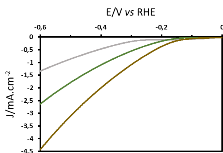
Figure 2. Polarization curves of 5 \times 10^{-4} mol L ^{-1} thio-POM PW _{11} -Mo _3 S _4 (brown), {Mo _3 S _4 } (green), and {PW _{11} } (grey) recorded on glassy carbon showing the highest efficiency of the hybrid {Mo _3 S _4 }-containing POM catalyst in 0.5 mol L ^{-1} aqueous sulfate solution pH = 1 (scan rate = 50 mV s ^{-1} ).
