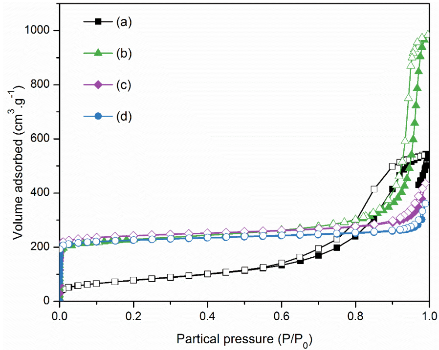
Fig. 4 Nitrogen sorption isotherms of amorphous precursor (a), FAU-1- nano (b), FAU-2- nano (c) and FAU-3- micron (d).
