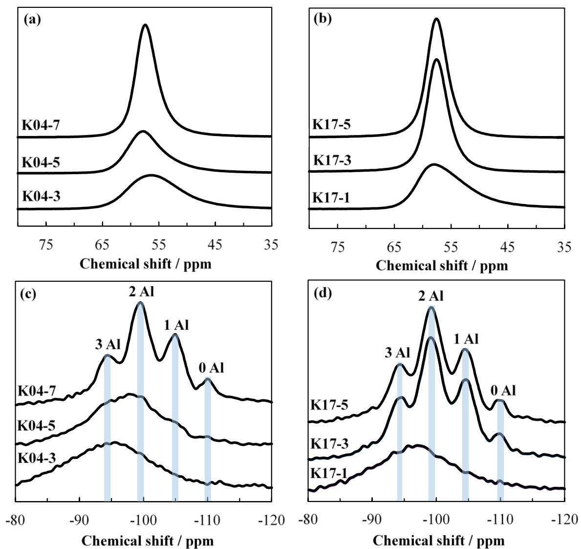
Figure 6. ^{27}\text{Al} MAS NMR spectra of the nanosized CHA samples (a) K04-3, K04-5, and K04-7, (b) K17-1, K17-3, and K17-5. ^{29}\text{Si} MAS NMR spectra of CHA samples (c) K04-3, K04-5, and K04-7, (d) K17-1, K17-3, and K17-5 of CHA samples.
