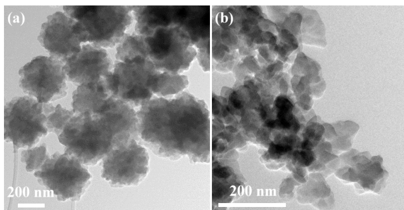
Figure 3. TEM images highlighting the morphology of fully crystalline nanosized CHA samples (a) K04-7 and (b) K17-3.
