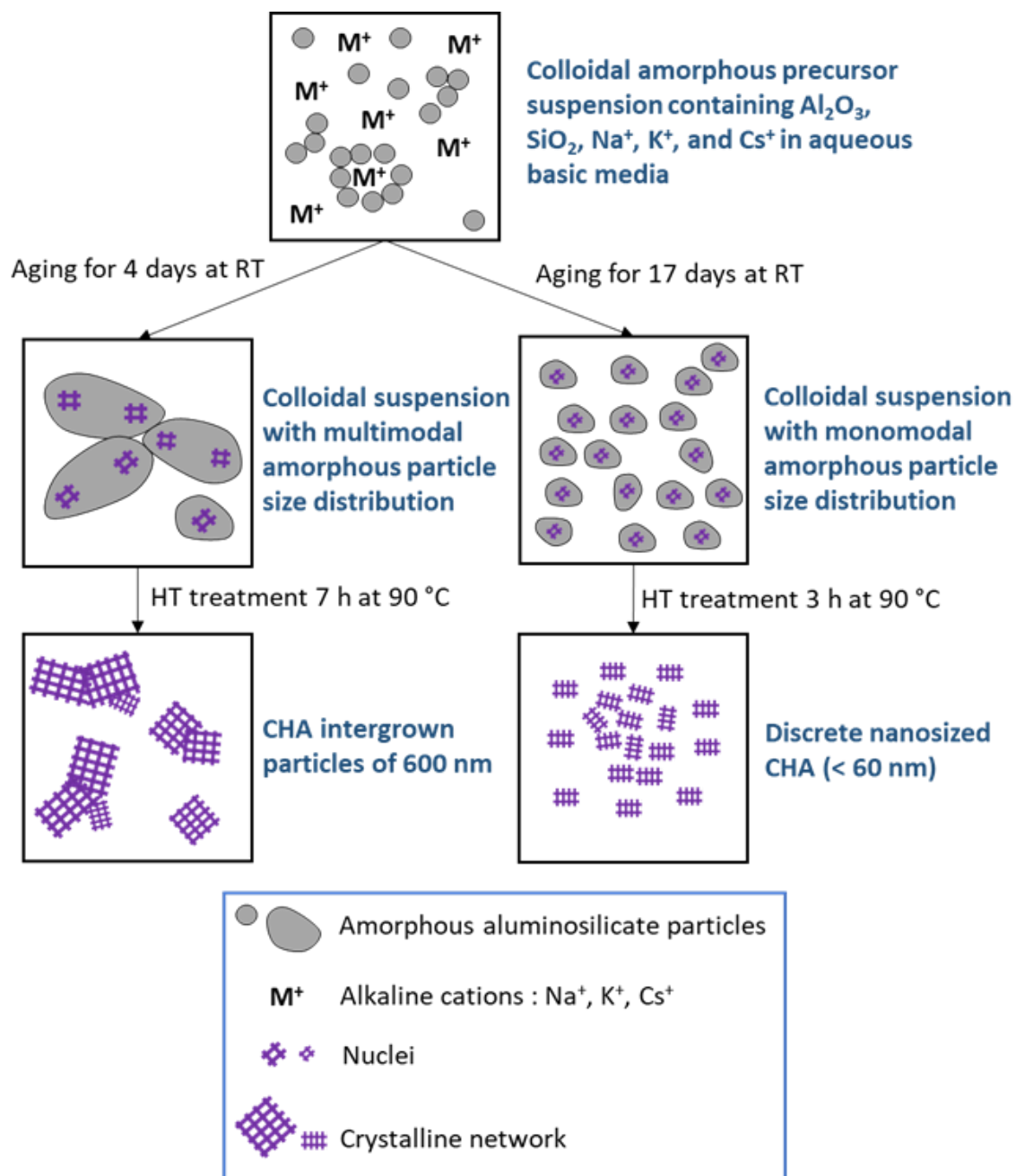
Scheme S1. Schematic illustration of the proposed crystallization pathway of nanosized CHA zeolite in colloidal precursor suspensions for series K04 and K17.
