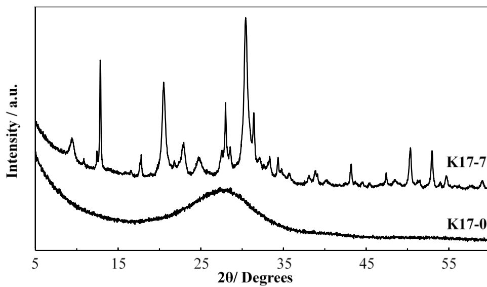
Figure S2. XRD patterns of the nanosized CHA from series K17: K17-0, and K17-7 samples.
