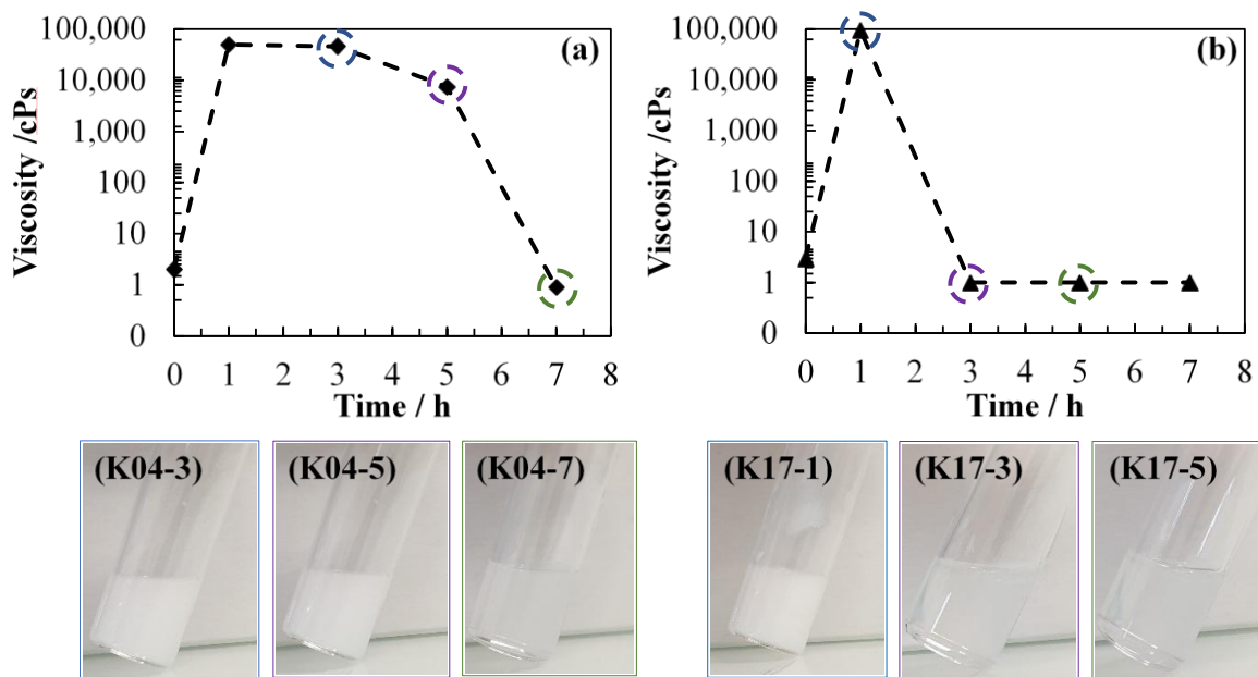
Figure 4. Top: viscosity changes of the colloidal precursor suspensions of samples from the series K04 and K17 at different times of hydrothermal treatment: (a) K04-0, K04-1, K04-3, K04-5, and K04-7, and (b) K17-0, K17-1, K17-3, K17-5, and K17-7. Bottom: pictures of the colloidal suspensions K04-3, K04-5, K04-7, K17-1, K17-3, and K17-5
