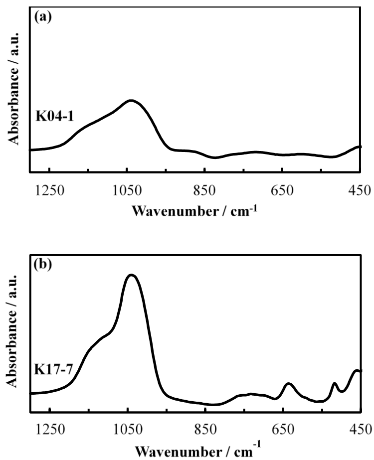
Figure S3. FTIR spectra of the nanosized CHA (a) K04-1 and (b) K17-7 samples.
