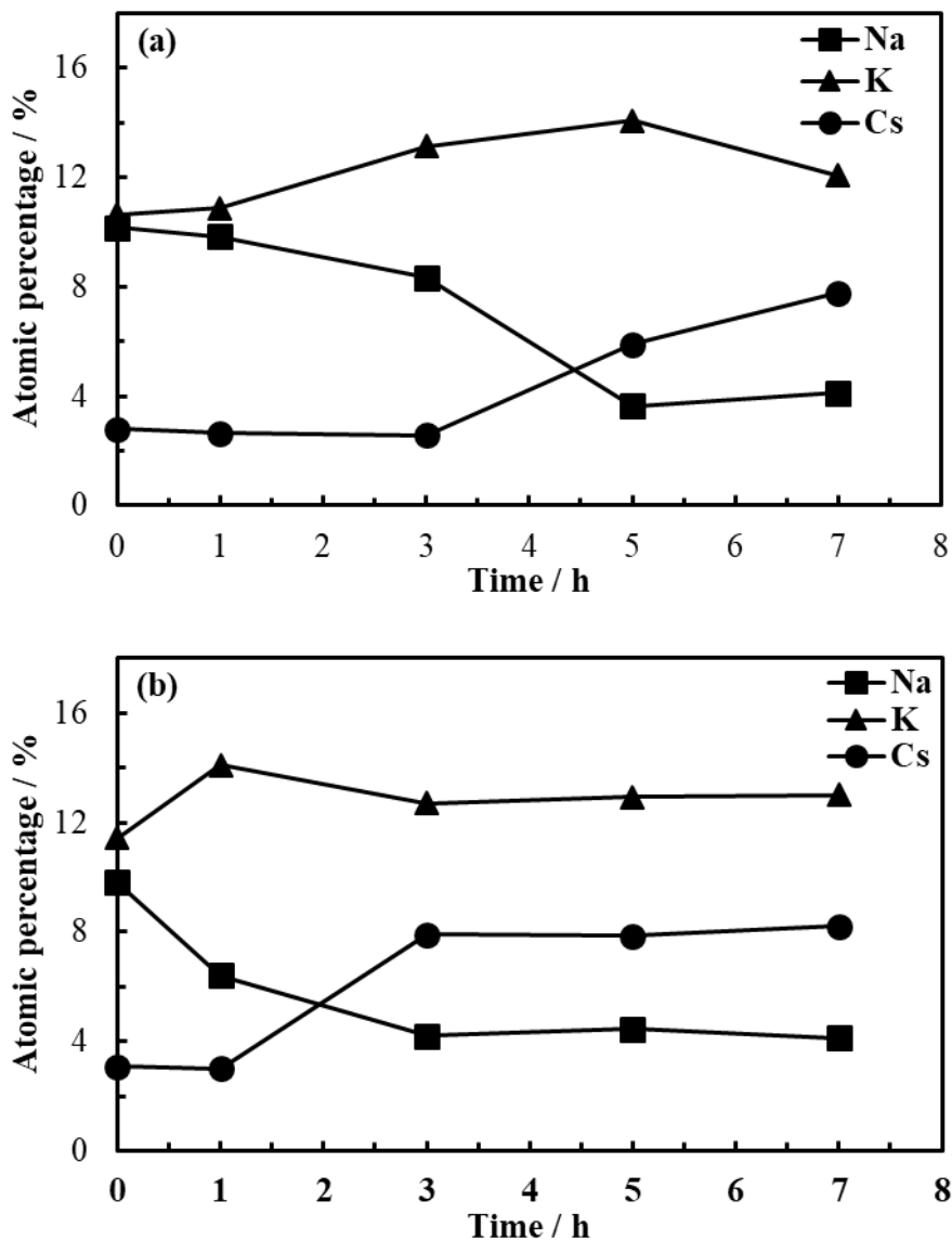
Figure 7. ICP-MS analysis revealing the change in the content of extra-framework cations ( \text{Na}^+ , \text{K}^+ , \text{Cs}^+ ) in the nanosized CHA series K04 and K17 at different times of hydrothermal treatment: (a) K04-0, K04-1, K04-3, K04-5, and K04-7, and (b) K17-0, K17-1, K17-3, K17-5, and K17-7.
