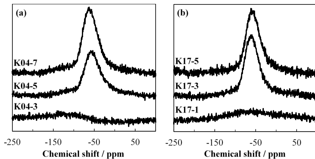
Figure S4. ^{133}\text{Cs} MAS NMR spectra of the nanosized CHA from (a) series K04: K04-3, K04-5, K04-7, and (b) series K17: K17-1, and K17-3 CHA, respectively.
