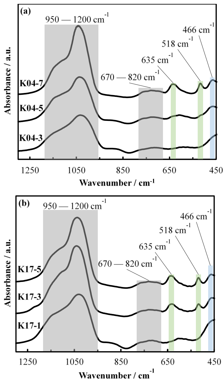
Figure 5. FTIR spectra of the nanosized CHA samples: (a) K04-3, K04-5, and K04-7 and (b) K17-1, K17-3, and K17-5 synthesized from colloidal precursor suspensions aged four and seventeen days, respectively.
