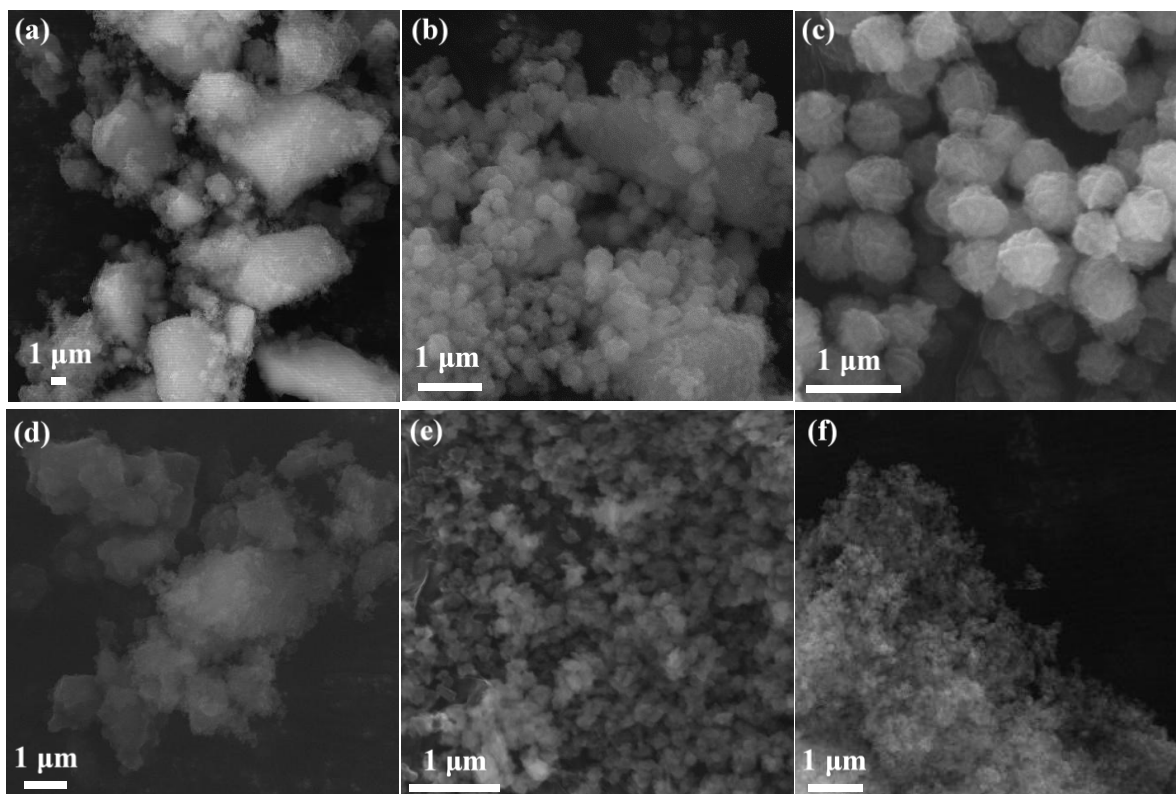
Figure 2. SEM images of the nanosized CHA samples (a) K04-3, (b) K04-5, and (c) K04-7 and samples (d) K17-1, (e) K17-3, and (f) K17-5 synthesized from colloidal precursor suspensions aged four and seventeen days, respectively.
