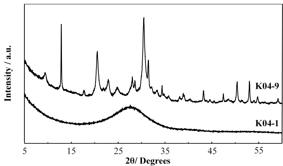
Figure S1. XRD patterns of the nanosized CHA from series K04: K04-1, and K04-9 samples.
