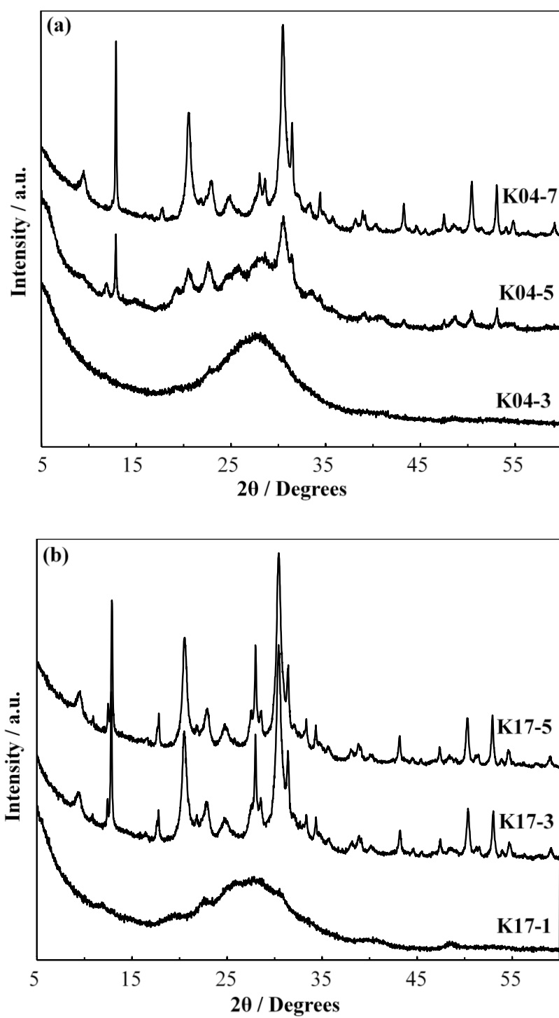
Figure 1. XRD patterns of the nanosized CHA samples (a) K04-3, K04-5, and K04-7 (b) K17-1, K17-03, and K17-5 synthesized from colloidal precursor suspensions aged four and seventeen days, respectively.
