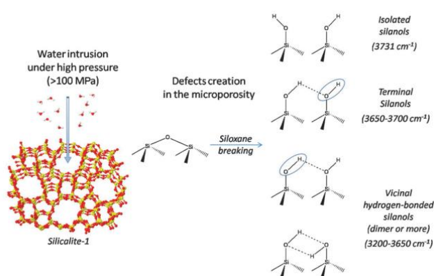
Fig. 17 Silanol formation in highly hydrophobic silicalite-1 synthesized in fluoride media during water intrusion. This figure has been reproduced from ref 106 with permission from Royal Society of Chemistry, copyright 2010.
