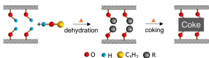
Fig. 24 Defect blocking mechanism promoted by coking in zeolite membranes.
