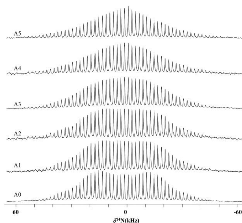
Fig. 6 Evolution of the ^{14}\text{N} spectra with the aluminium loading in a series of as-synthesized ZSM-5 zeolites. This figure has been reproduced from ref 45 with permission from American Chemical Society, copyright 2017.
