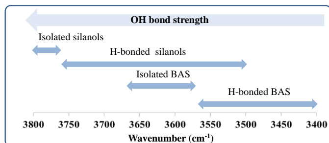
Fig. 3 Characteristic stretching frequency of OH bonds in zeolites
