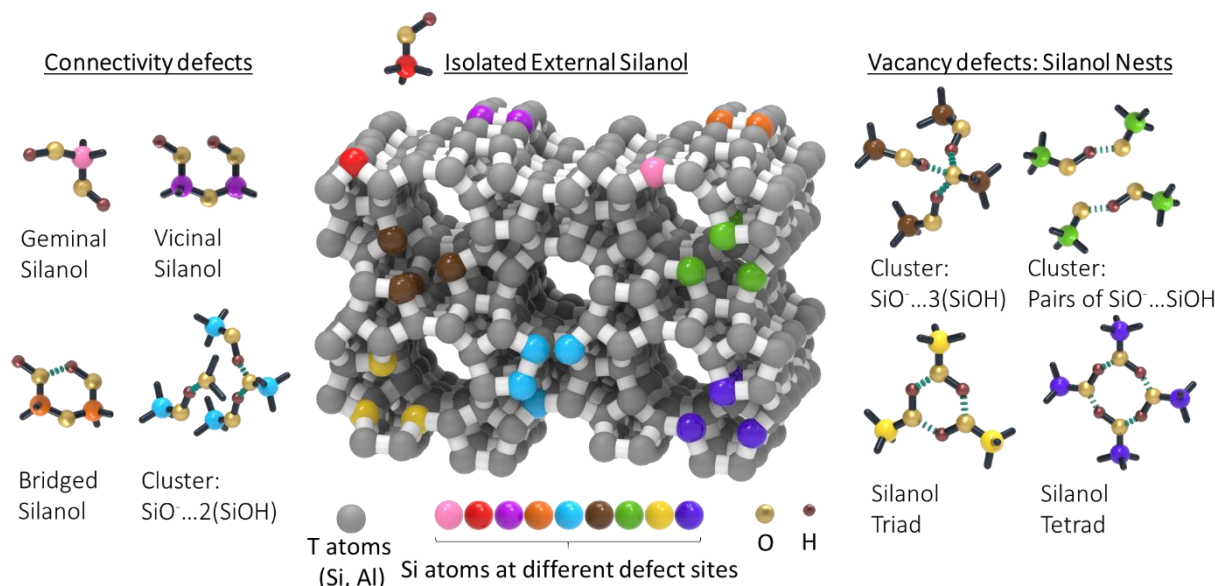
Fig. 1 Schematic representation of different types of silanols grouped into three main categories: isolated external silanols, connectivity defects and vacancy defects. Green dotted lines indicate hydrogen bonding.
