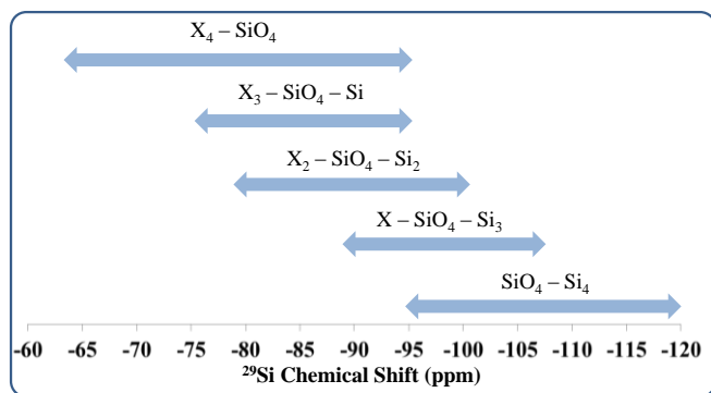
Fig. 4. Characteristic ^{29}\text{Si} chemical shifts in zeolites
