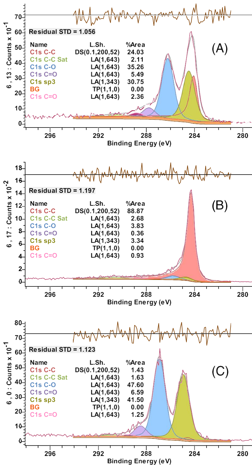
FIGURE 3 Representative narrow scans from the image in Figure 2 that correspond to (A) a mixture of GO and reduced GO, (B) fully reduced GO, and (C) GO. These peak models all make use of the same components, line shapes, and constraints, as defined in Table 1. The first numbers on the vertical axis label represent pixels (the location of the spectra in the image). TP corresponds to a trapezoidal component that represents background intensity in CasaXPS 30
