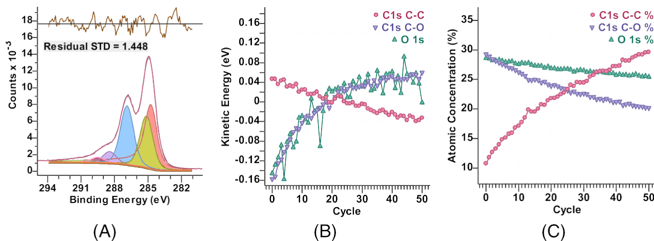
FIGURE 6 (A) Spectrum of GO/reduced-GO obtained at a pass energy of 40 and an analysis area of 200 \mu\text{m} that was fitted with the peak model in Figure 3 after relaxing the interval constraints for FWHM in Table 1. (B) Plot of the offset in kinetic energy from the mean component positions for C 1s C-C and C 1s C-O combined with a similar energy offset from the mean calculated for the O 1s signal measured via signal relative to a Shirley background. (C) Relative intensities for the C 1s C-C and C 1s C-O components together with the O 1s intensity converted to atomic concentrations using Scofield cross-sections, 35 effective attenuation lengths, 36 and the Thermo K-Alpha+ transmission correction
