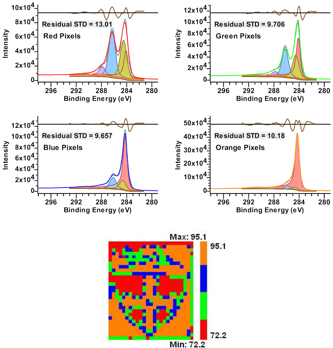
FIGURE 5 The peak model used in Figure 3 was applied to the data represented in Figure 2. The resulting, colored pixels shown here were obtained/derived from the spatial zones within the image. Red indicates a region in which GO is the dominant material, while orange indicates where rGO is predominantly found. Pixels representing the interface between GO and rGO are marked with green and blue
