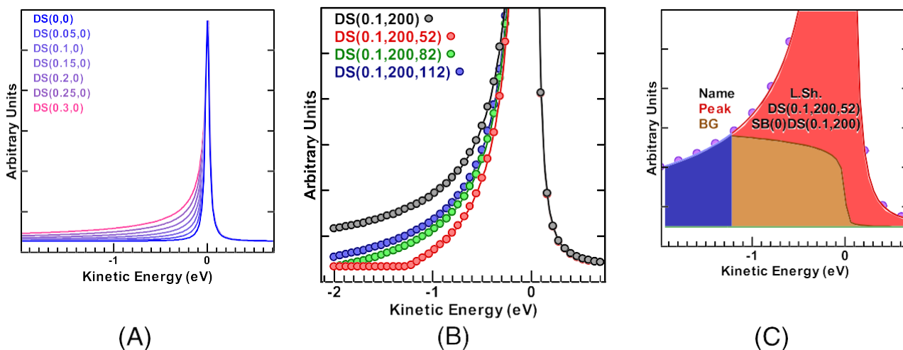
FIGURE 1 (A) A series of DS line shapes corresponding to DS(0, 0) (a pure Lorentzian) to DS(0.3, 0) (a pure Doniach Sunjic with substantial asymmetry). Line shapes are displayed normalized to their maximum intensity values. (B) DSS line shapes with different values of l , which is defined in Equation 9. Line shapes are displayed normalized to their maximum intensity values. (C) DS(0.1, 200) line shape (purple dots) with Shirley response beneath. When the Shirley response (brown area) is subtracted from the DS(0.1, 200) line shape, the DS(0.1, 200, 52) line shape is created, which corresponds to the red area in Figure 1A and the peak shape defined by the red dots in Figure 1B. This process excludes the blue area from the DS(0.1, 200, 52) line shape. The point at which the Shirley background touches the DS(0.1, 200) line shape corresponds to the parameter l in Equation 8
