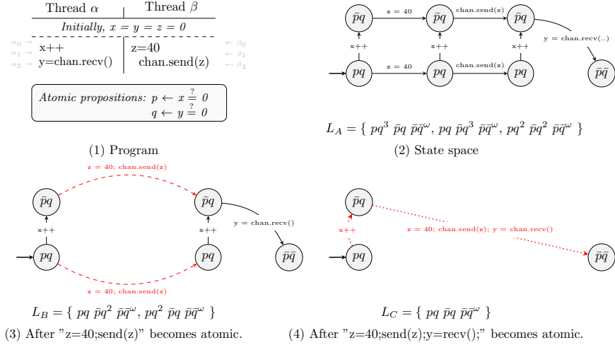
Fig. 1: Example of reductions. (1) describes a program composed of two threads and 3 integer variables. The chan variable designates a communication channel where send(int) insert a message and int recv() consumes a message with a blocking semantic if the channel is empty. We consider that the logic only observes whether x or y is zero noted p and q . (2) depicts the state-space represented as a Kripke structure. Each node is labelled by the value of atomic propositions p and q . When an instruction is executed the value of these propositions may evolve. (3) represents the state-space of (1) if actions of thread \beta " z = 40; chan.send(z); " are fused into a single atomic operation. (4) represents the state-space of (1) after further considering that the three actions of the original program " z = 40; chan.send(z); y = chan.recv(); " are now a single atomic step.
