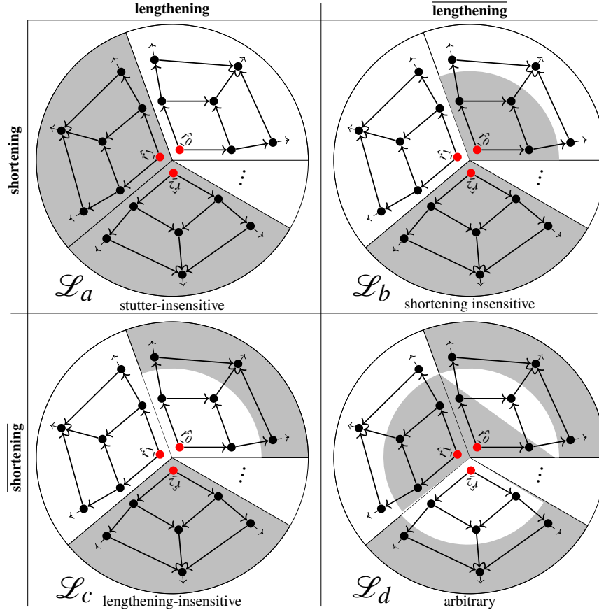
Fig. 2: \Sigma^\omega is represented as a circle that is partitioned into equivalence classes of runs (\hat{r}_0, \hat{r}_1 \dots) . Each point in the space is a run, and some of the \leq relations are represented as arrows; the red point is the shortest run \hat{r} in the equivalence class. Gray areas are inside the language, white are outside of it. Four languages are depicted:
