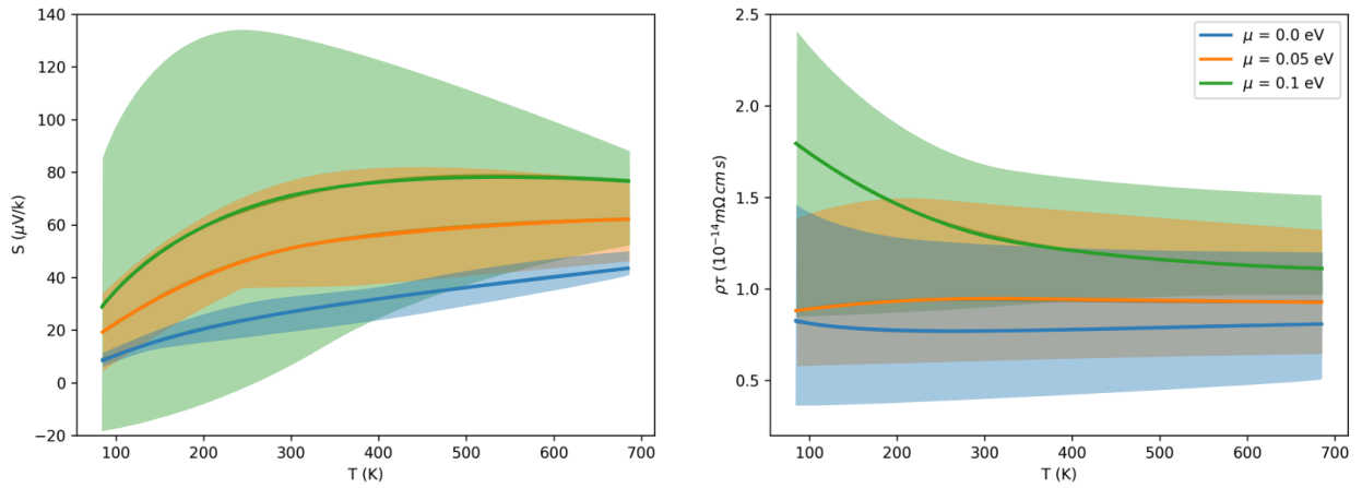
Figure 9. Seebeck coefficient (left) and electrical resistivity (right, multiplied by the constant relaxation time \tau ) as a function of temperature. The three curves correspond to three different doping levels ( E_F = \mu = 0.0 eV is the theoretical value for \text{Cu}_{22}\text{Sn}_{10}\text{S}_{32} and is used as energy reference). In the rigid band approximation, shifting up the chemical potential is equivalent to remove holes from the system. We used three different models to simulate disorder: the shaded regions indicate the dispersion of the transport coefficients as the model to represent the Cu-Sn disorder changes; the solid lines indicate the averages.
