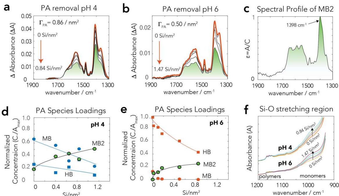
Figure 8. ATR-FTIR spectra and chemometric (MCR) analyses of N 2 -dry (298 K) goethite initially equilibrated in 50 m 2 /L suspensions in 10 mM NaCl at 298 K (cf. Figure S8 for uncorrected spectra). (a–b) Spectra at pH (a) 4 and (b) 6 at various PA loadings with 100 μM PA and 0–1000 μM Si. Note that combination (1662 cm -1 ) and overtones (1789 cm -1 ) of Fe-O-H bending modes (Figure S8) were removed. Decreased PA loadings result from the competitive binding of silicate at these fixed pH values. (c–e) Chemometric analyses used concentration profiles of HB and MB of Figure 7 to also extract (c) the spectral profile of a new component PA-Si. The associated concentration profiles of these three species reveal the predominant removal of (d) MB species at pH 4 but of (e) HB species at pH 6. Lines in (d) and (e) are only visual guides. (f) Si-O stretching region in corresponding spectra of (a) and (b), showing preferential appearance of monomeric silicate species.
