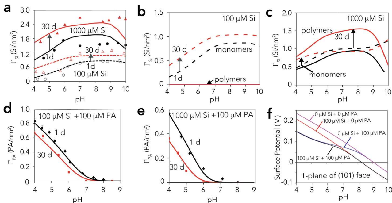
Figure 6. Batch adsorption data and SCM modeling. (a-c) Silicate loadings, (d-e) PA loadings, and (f) surface electrostatic potentials achieved in suspensions of 50 \text{m}^2/\text{L} goethite in 10 mM NaCl at 298 K. (a-e) Comparison of experimental and predicted SCM loadings achieved at 1 d (black) and 30 d (red) of equilibration time in competitive systems with total concentrations of 100 \mu\text{M} PA with (a, b, d) 100 or (a, c, e) 1000 \mu\text{M} silicate. (f) Predicted surface potentials of the 1-plane of the (101) face of goethite, containing unbound silicate oxo groups and carboxyl groups of HB PA species (Table 1; cf. Figure S6 for full modeling results).
