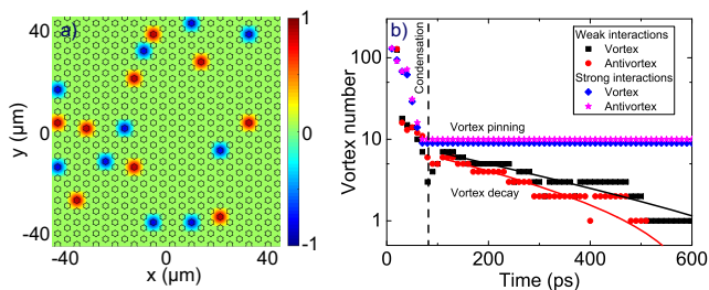
FIG. 2: a) Spatial image of the curl of the wavefunction after condensation exhibiting topological defects. The lattice potential is shown as a black line. b) The number of topological defects as a function of time in the case of strong ( gn = 1 meV) and weak ( gn = 0.25 meV) interactions (points - pinned and free vortices, respectively). Solid lines show exponential decay fits.
