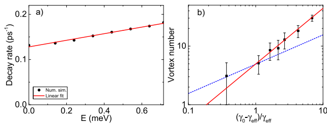
FIG. 3: (a) Effective decay rate scales linearly with mode energy (circles – numerical simulation, solid line – linear fit). (b) Density of topological defects as a function of the quenching parameter (effective pumping) and a power law fit with a scaling exponent 0.95 \pm 0.05 .
