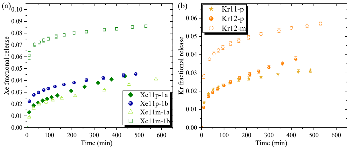
Fig. 3 – Cumulated release fractions of (a) 800 keV Xe and (b) 500 keV Kr from low fluence samples ( \leq 2 \times 10^{12} i/\text{cm}^2 ) ( 1300^\circ\text{C} annealings).
