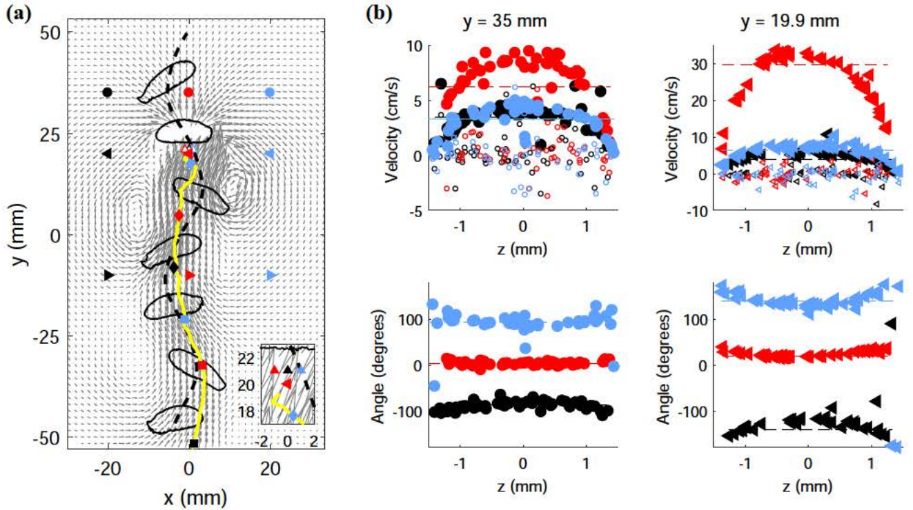
Fig. 11 Velocity profiles measured across the gap at various locations for a given time step corresponding to t = 0.6 s. The particles inside squares of side 1.286 mm in the (x, y) plane and for all values of z were considered. The bubble centroid is at (x, y) = (-1.5, 25.1) mm at that instant. a Positions where the velocity profiles were measured; the trajectory of the bubble is shown as a dashed line, as well as its contour at regular time intervals \Delta t = 0.0714 s in black continuous lines; the yellow line is the line of maximum velocity x_{v_{\max}}(y, t) at the
