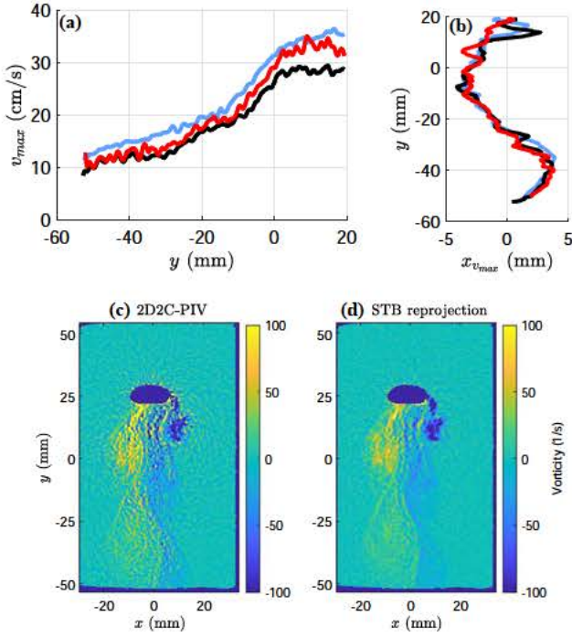
Fig. 9 Consistency of wake characterization using velocities averaged through the gap obtained from the STB reprojection (black line) and from 2D2C-PIV measurements using the front projections of the tomographic reconstruction (red line). a Longitudinal evolution of the norm v_{\max} , b position of the line where v_{\max} is detected, c vorticity field obtained from 2D2C-PIV measurements, d vorticity field obtained from STB reprojection. (in a and b light blue lines represent the measurements from the STB reprojection using only a central slice of thickness \delta z = 0.4 mm)
