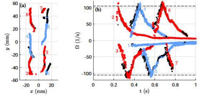
Fig. 10 Released vortex characterization from velocities averaged through the gap obtained either from 2D2C-PIV measurements or STB reprojection. a Trajectories of the released vortices, b temporal evolution of the vorticity of the released vortices. Black filled symbols: STB, red or light blue open symbols: PIV, dashed line is the value provided by the scaling law for \Omega_0 from Filella et al. (2015). Vortices were numbered following the order of release from the bubble surface. Only 3 vortices were tracked for sufficiently long times as to finally reach a fixed position
