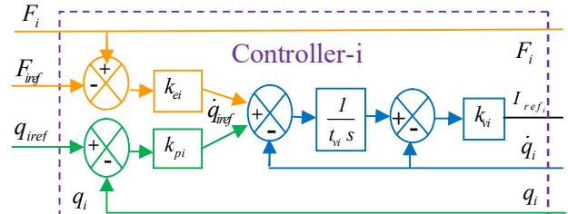
Fig. 4 Controller of speed, position and force of robot- i
