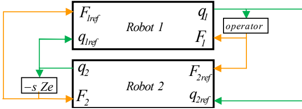
Fig. 5 Four-channel bilateral teleoperation system
