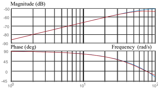
Fig. 10 h_{22}=1/Z_{ai} Bode diagram (PP)
