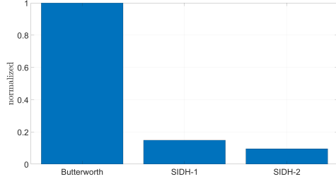
Fig. 7. Evaluation of the normalized index SSE for h_1 = 2 \cdot 10^{-4} s.
