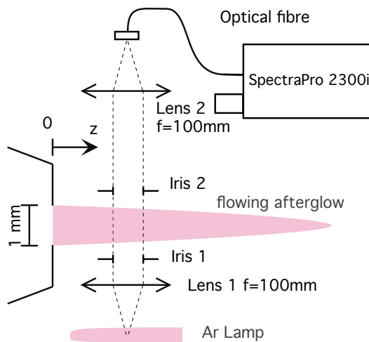
Figure 3. Schematic diagram of the optical absorption spectroscopy setup.
