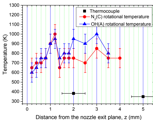
Figure 7. Axial distribution of the rotational temperature of OH(A) and N 2 (C) obtained using Speicair and gas temperature measured with a thermocouple, at 5 L/min of Ar and 40 W.
