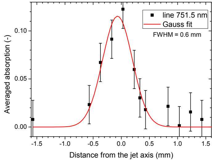
Figure 5. Radial profile of the absorption for the 751.5 nm line, 1 cm away from the nozzle exit plane.
