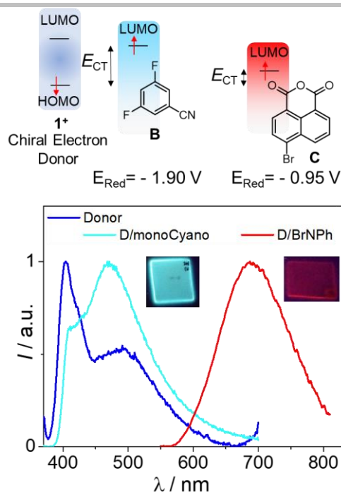
Figure 5. Top: Chemical structures of the different electron acceptors screened in this study to obtain multi-colored chiral exciplex luminescence with the associated reduction potentials, and bottom: exciplex luminescence spectra recorded at 298 K of spin-coated films involving chiral 1 as the donor and 3,5-difluorobenzonitrile ( B , sky blue), and 4-bromonaphthalene monoanhydride ( C , red) electron acceptor units, with associated pictures.
