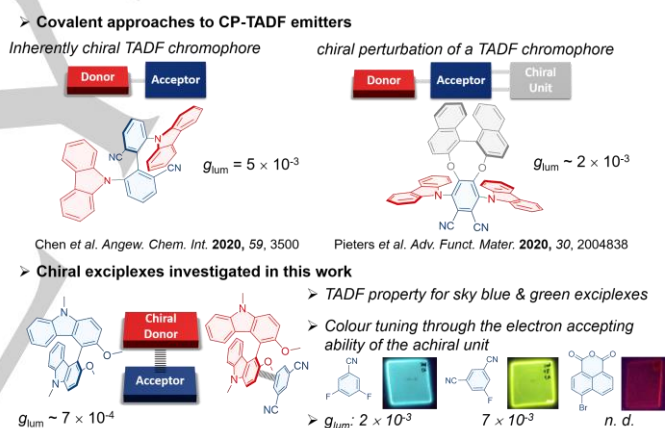
Figure 1. Top: Current molecular designs of CP-TADF emitters. Bottom: chiral luminescent exciplex approach investigated in this report (n.d.: not detected).
