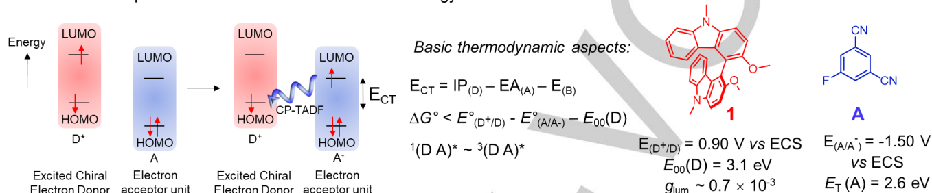
Figure 2. Illustration of the circularly polarized luminescence process obtained in the reported chiral exciplexes with basic thermodynamic considerations regarding the HOMO and LUMO of the respective donor and acceptor neutral ground-states, respectively. E_{CT} , the energy of the charge-transfer process with IP = ionization potential, EA = electron affinity and E_B , the binding energy of the charge-transfer state. [10] \Delta G^\circ is the driving force for the photoinduced electron transfer between the donor and the acceptor implying the oxidation and reduction potentials of the donor and acceptor, respectively, and E_{00} the optical gap of the donor molecule. Chemical structures of the chiral electron donor and the achiral electron acceptor investigated as luminescent exciplexes.
