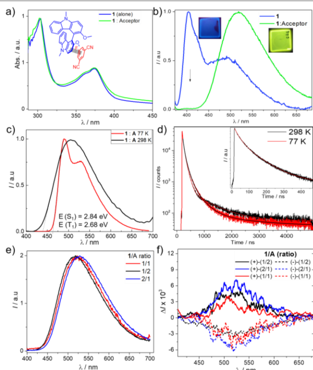
Figure 3. a) and b) UV-vis absorption and luminescence spectra, respectively, of 1 alone (blue solid line) and 1 blended (exciplex) with 5-fluoroisophthalonitrile (green solid line) from spin-coated film substrate excited at 370 nm; c) Exciplex luminescence spectra recorded at 77 K (recorded with a 10 ms delayed time, red solid line) and 298 K (black solid line), with estimated values of the singlet and triplet excited-states; d) Corresponding luminescence decays of exciplex recording at 77 K (red solid line) and 298 K (black solid line) with an inset focusing on the short lifetime decays (see details in Figure S10); e) and f) luminescence and CPL spectra, respectively, of exciplexes involving different ratios of Donor and Acceptor compounds.
