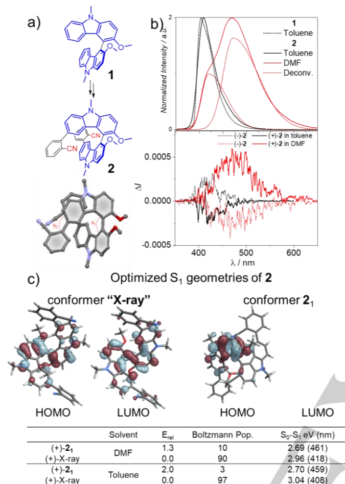
Figure 4. a) XRD structure of 2 and precursor 1 and b), emission (only the emission of (+)- 2 is shown) and CPL spectra of (+)- and (-)- 2 in toluene (black lines) and DMF (red lines) at 298 K (the normalization is done to 2 to have a direct lecture of the g lum value at the emission maxima of 2 ). Deconvolution (Deconv.) of the emission of compound 2 in DMF (red dotted lines), with bands found at 418 and 478 nm; c) Isosurfaces ( \pm 0.035 au) of the frontier molecular orbitals (HOMO/LUMO classification according to the ground state) for optimized structures of conformers of (+)- 2 (X-ray and 2 1 ) in DMF (see SI for details), relative conformer energy (in kcal·mol -1 ) in toluene and DMF solvents, Boltzmann weight at 298 K (in %) and first electronic transition in the excited state optimization in solution in eV (nm), all obtained using the TD-DFT/PBE0/def2-SV(P)/D3 method.
